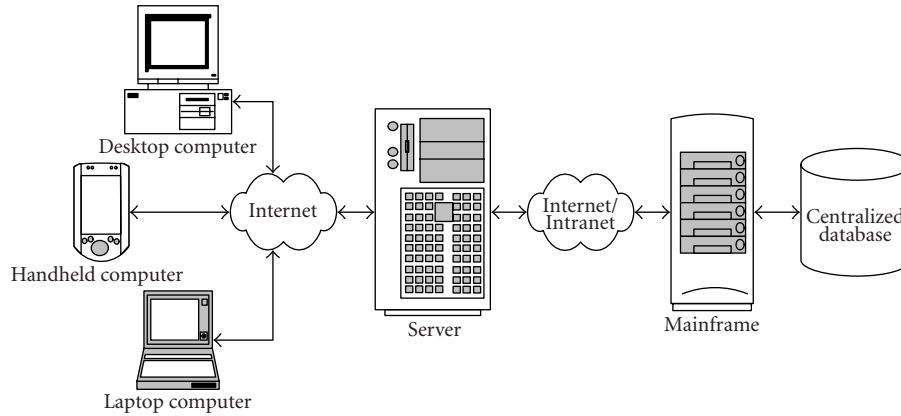
FIGURE 1: Client-server architecture.
