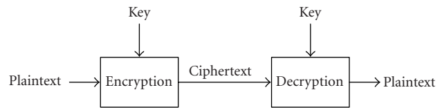
FIGURE 4: Encryption/decryption process.
