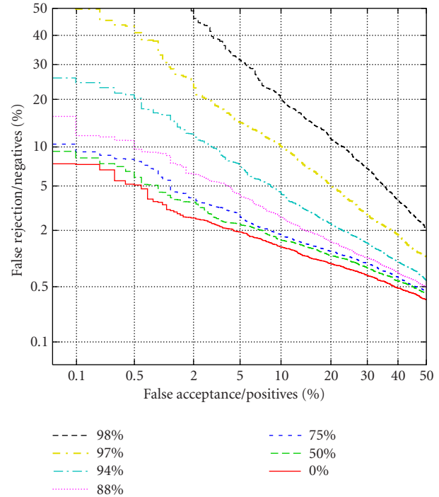
FIGURE 8: Speaker verification performance for varying degrees of feature vector loss, from 0 up to 98% (with a minimum of 2 feature vectors maintained in all tests) for 4-digit string tests.
