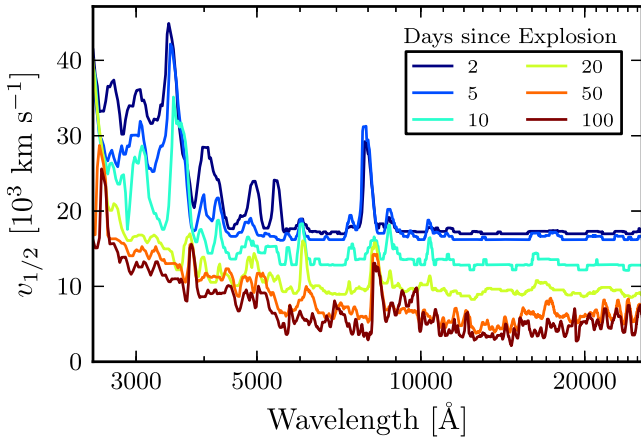
Figure 3. Illustration of the wavelength dependence of the spectrum-formation region, represented here using the velocity above which 50 per cent of the flux at a given wavelength is emitted. This velocity is computed based on equation (3), but replacing the wavelength-averaged flux contribution \overline{\delta F(v)} of equation (2) with the non-averaged \delta F(r, \lambda, t) of equation (1).
