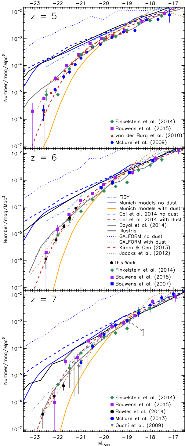
Figure 12. A comparison of the latest observational data on the rest-frame UV galaxy LF at z \simeq 5, 6 and 7 (including the new results on the bright end presented here and in Bowler et al. (2014)) with the predictions of several of the latest semi-analytic and hydrodynamical models of galaxy formation. The sources of the data points are indicated in each panel, with the various model references provided in the central ( z \simeq 6 ) panel. The implications of this comparison are discussed in the text (Section 8.3) but in general it can be seen that most of the models struggle to reproduce the observations over the redshift range z \simeq 5-7 when faced with the large dynamic range now made possible by the combined ground-based and HST data set. See the text for full references to the models displayed here.
