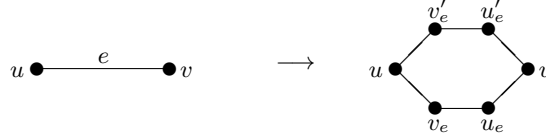
Fig. 1. Replacement of an edge by two paths
