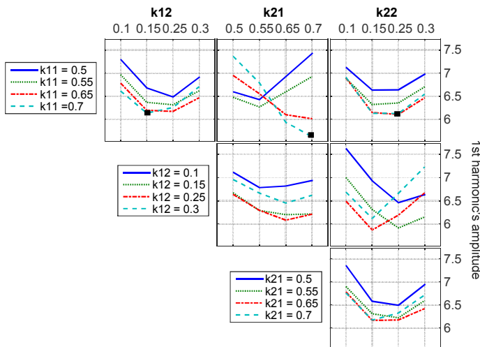
Fig. 21. Results of the DOE for the 1 st harmonic' amplitude
