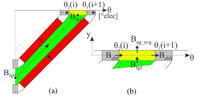
Fig.7 Flux density mean path in a rotor flux-guide (a). Local saturation near the exterior iron bridge (b)
