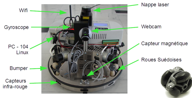
FIGURE 1 – Robot mobile Robotino
