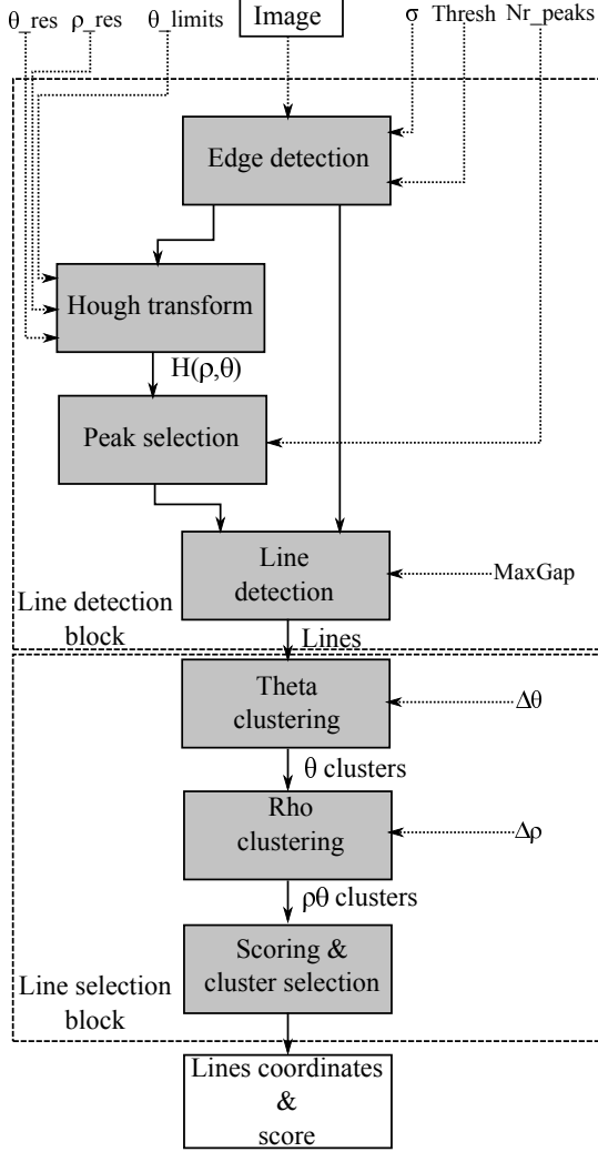
Fig. 1. Algorithm general scheme. Dotted lines indicate input data.
