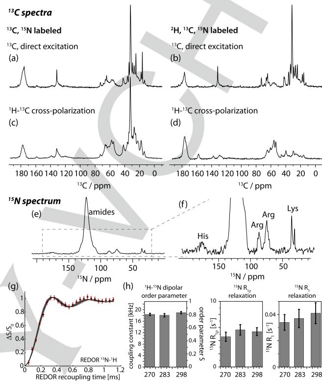
Figure 2. 1D NMR characterization of nanodisc-embedded CzcD. ^{13}\text{C} and ^{15}\text{N} solid-state NMR spectra of [\text{C}^{13}, \text{N}^{15}] - (a, c, e, f) and [\text{C}^{13}, \text{N}^{15}] -labeled (b, d) CzcD in native nanodiscs, recorded at 55 kHz MAS frequency at 14.1 T static magnetic field strength (600 MHz ^1\text{H} Larmor frequency). (g) REDOR measurement of the bulk ^1\text{H} - ^{15}\text{N} dipolar order parameter. A single fit parameter, the effective coupling constant, is invoked in this fit. (h) Fitted parameters of dipolar couplings, the order parameters derived from the dipolar couplings, and ^{15}\text{N} relaxation rate constants. Further details are provided in Fig. S8.
