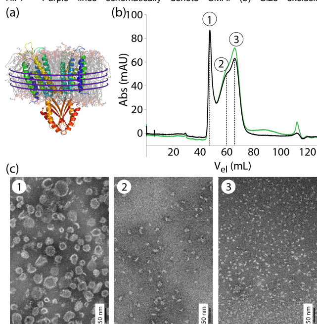
Figure 1. (a) Model of CzcD in a nanodisc, based on a homology model using YiiP. [18] Purple lines schematically denote SMA. (b) Size exclusion
