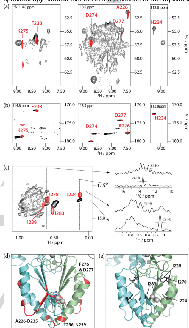
Figure 3. Proton-detected 3D (a,b) and 2D (c) spectra of nanodisc-embedded deuterated CzcD, (a) hCANH and (b) hCONH correlation spectrum of [\text{2H}, \text{13C}, \text{15N}] CzcD obtained at 600 MHz ^1\text{H} Larmor frequency and 55 kHz MAS frequency. In addition to the ssNMR spectra, shown in black, solution-state spectra of the soluble domain are overlaid (red). Further views of these spectra are provided in Fig. S9. (c) 2D ssNMR HC spectrum of [\text{2H}, \text{12C}] Ile- \delta 1 - [\text{13CH}_3] CzcD (black) and solution-state ^{13}\text{C} -HSQC (red) on [\text{13C}, \text{15N}] soluble domain. In all cases, the soluble domain spectra were obtained on a sample containing a two-fold molar excess of \text{Zn}^{2+} . (d) Location of the residues identified in the 3D spectra of panels mapped on the YjiP crystal structure (a, b). (e) Localization of the Ile side chains in the cytoplasmic domain within a CzcD homology model.
