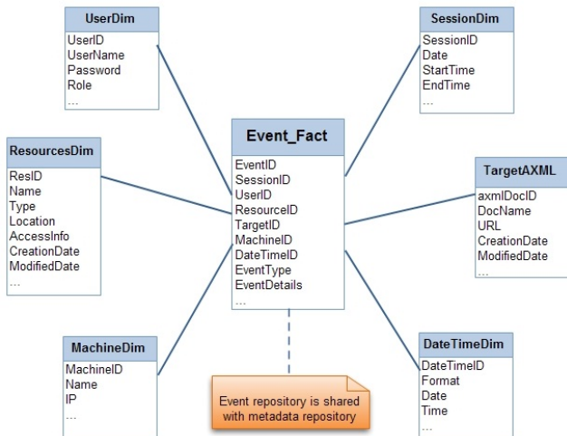
Fig. 8 Logical star schema of event repository
