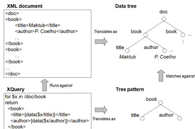
Fig. 1. Tree representation of XML documents and queries
