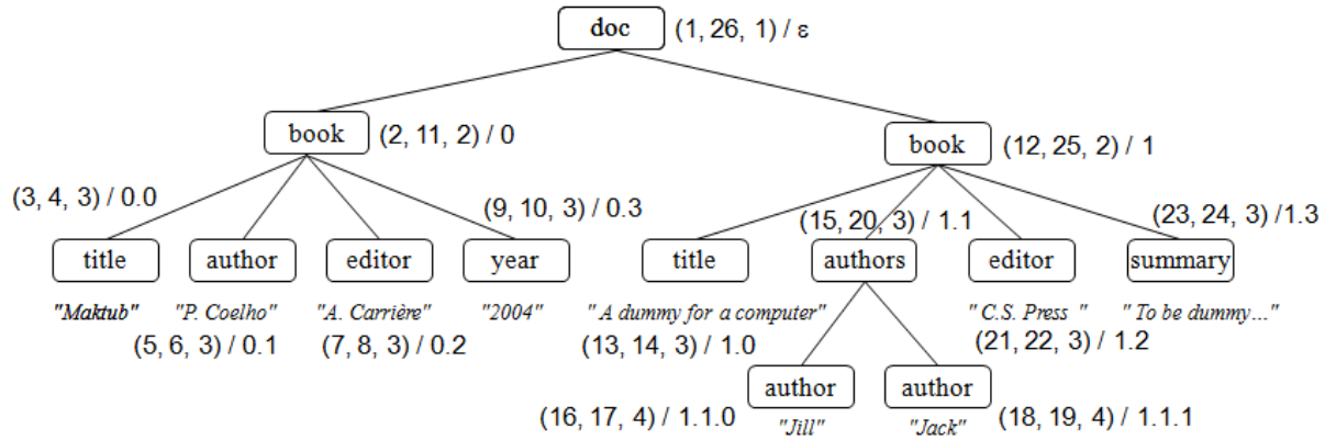
Fig. 11. Sample data tree labeling
