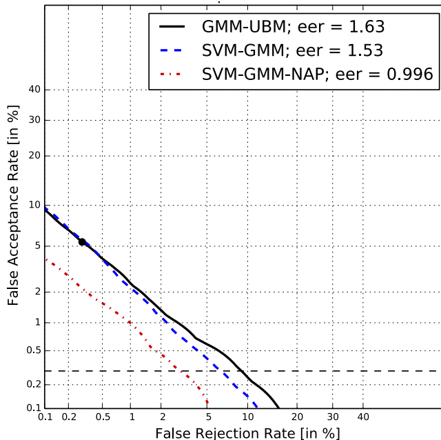
Fig. 1: DET curve on the male impostor-correct condition of RSR2015 protocol Part I.
