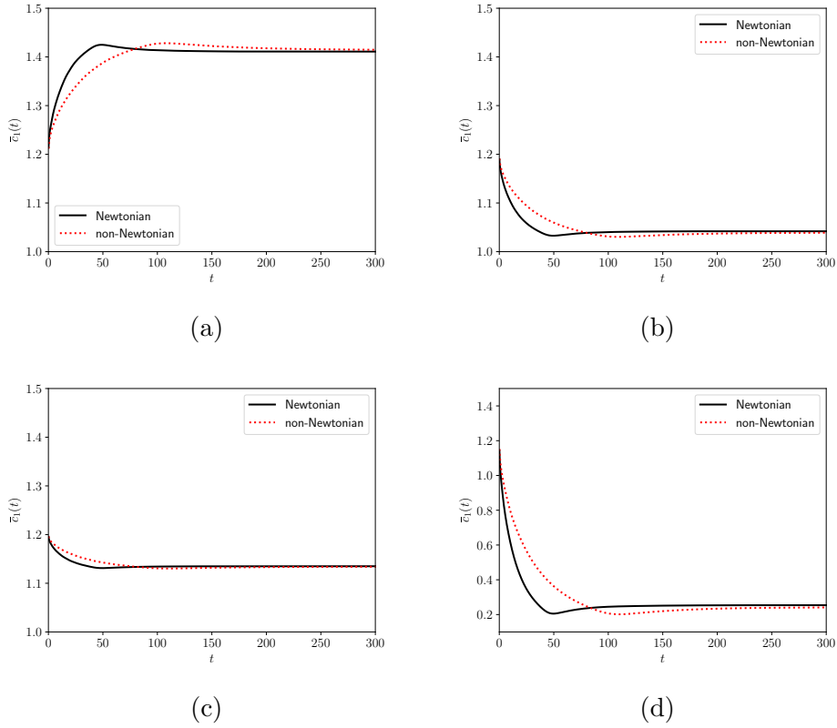
Figure 8: Evolution of the concentration \bar{c}_1(t) (in mol.m -3 or, equivalently, in mmol.l -1 ) of the free calcium in the blood at the exit of the dialyzer for dialysate fluids described in Table 6. (a) Dialysate \mathcal{D}_0 . (b) Dialysate \mathcal{D}_1 . (c) Dialysate \mathcal{D}_2 . (d) Dialysate \mathcal{D}_3 .
