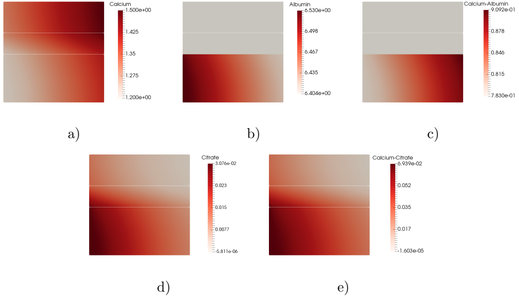
Figure 7: Concentrations c_i (in \text{mol}\cdot\text{m}^{-3} or, equivalently, in \text{mmol}\cdot\text{l}^{-1} ) in the domain \omega at a non-dimensional time T^* corresponding to approximately 300 s, for (EX1) and dialysate \mathcal{D}_0 : a) calcium. b) free albumin binding sites for calcium. c) calcium-albumin sites. d) citrate. e) calcium-citrate.
