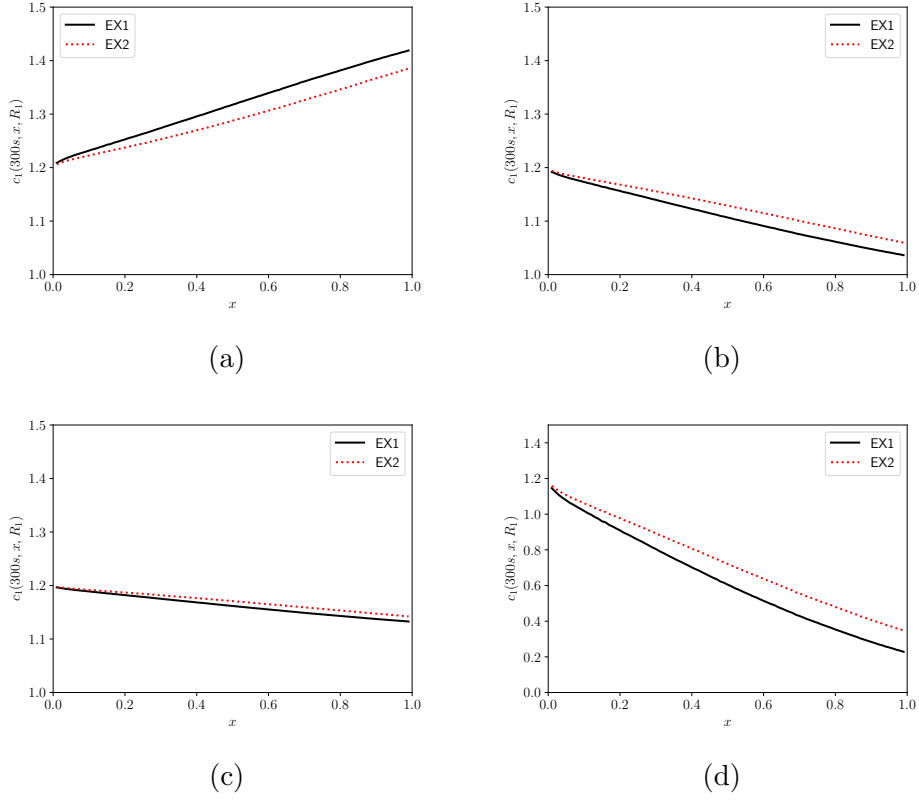
Figure 10: Longitudinal distribution of the concentration \bar{c}_1(t) (in \text{mol}\cdot\text{m}^{-3} or, equivalently, in \text{mmol}\cdot\text{l}^{-1} ) of free calcium in the blood at the blood/membrane interface at time 300 s for dialysate fluids described in Table 6. (a) Dialysate \mathcal{D}_0 . (b) Dialysate \mathcal{D}_1 . (c) Dialysate \mathcal{D}_2 . (d) Dialysate \mathcal{D}_3 .
