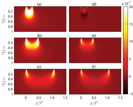
Fig. 2. Matrix elements of the dimensionless sensitivity kernel (\ell^*)^2 K for normal incidence and normal detection. The matrix element K_{11} is shown in Panels (a-c) and the linear combination K_{41} + K_{44} is shown in panels (d-f). From top to bottom, the source-detector separation is 0.225\ell^* , 0.45\ell^* and 1.05\ell^* .
