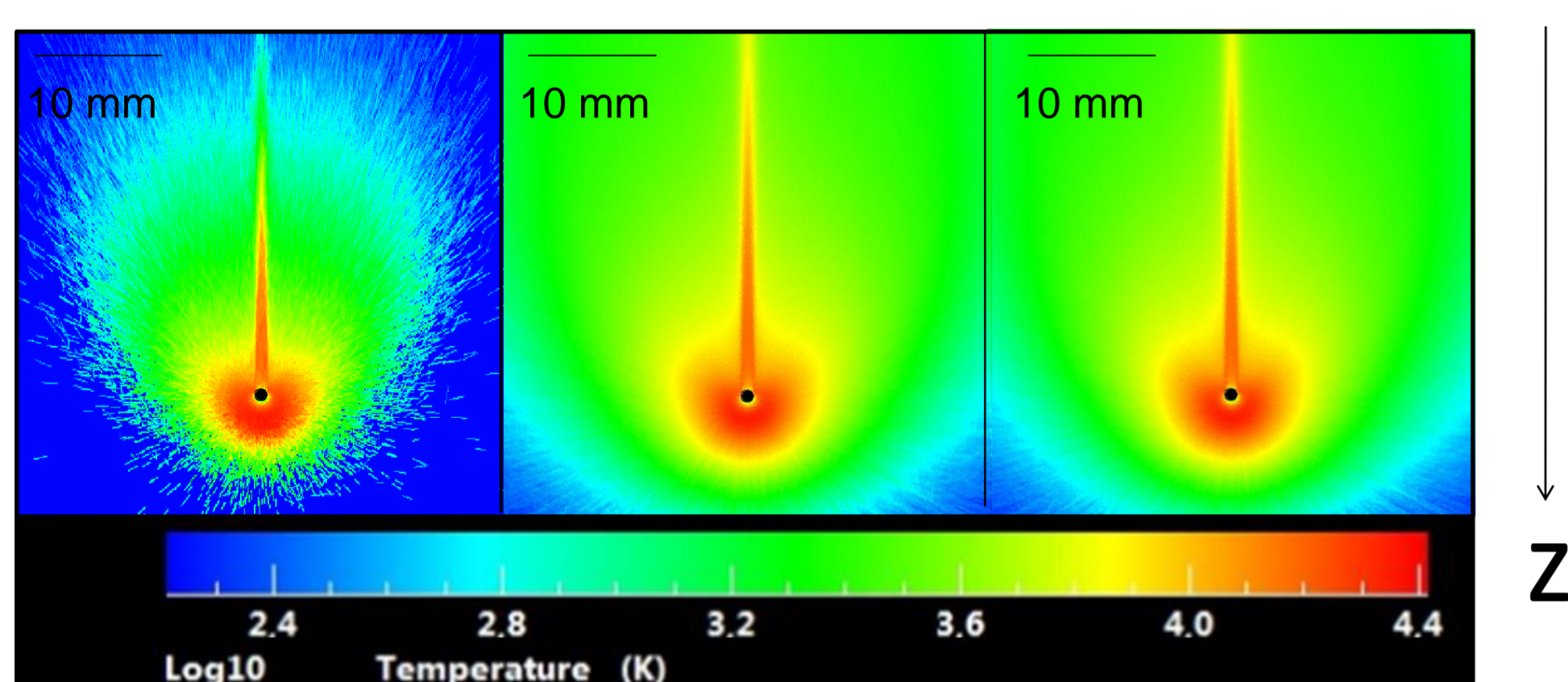
Figure 1: Simulation evolution until steady state reached.
