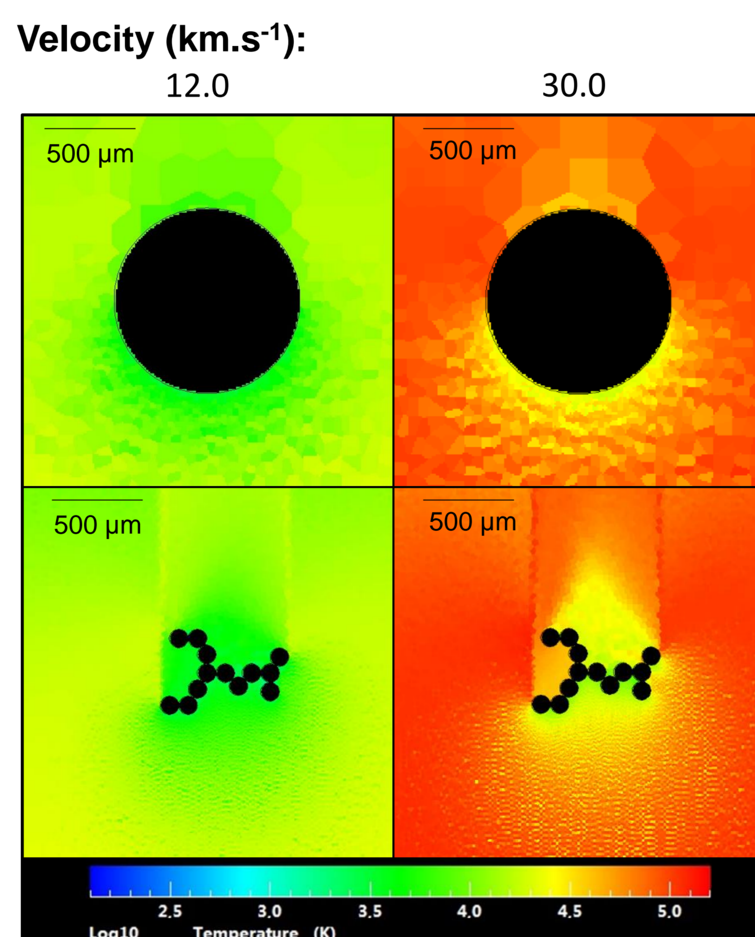
Figure 3: Comparison between atmospheric entry of a 1 mm diameter sphere and a fractal aggregate of 13 grains of 0.05 mm each (zoom on the particle)
