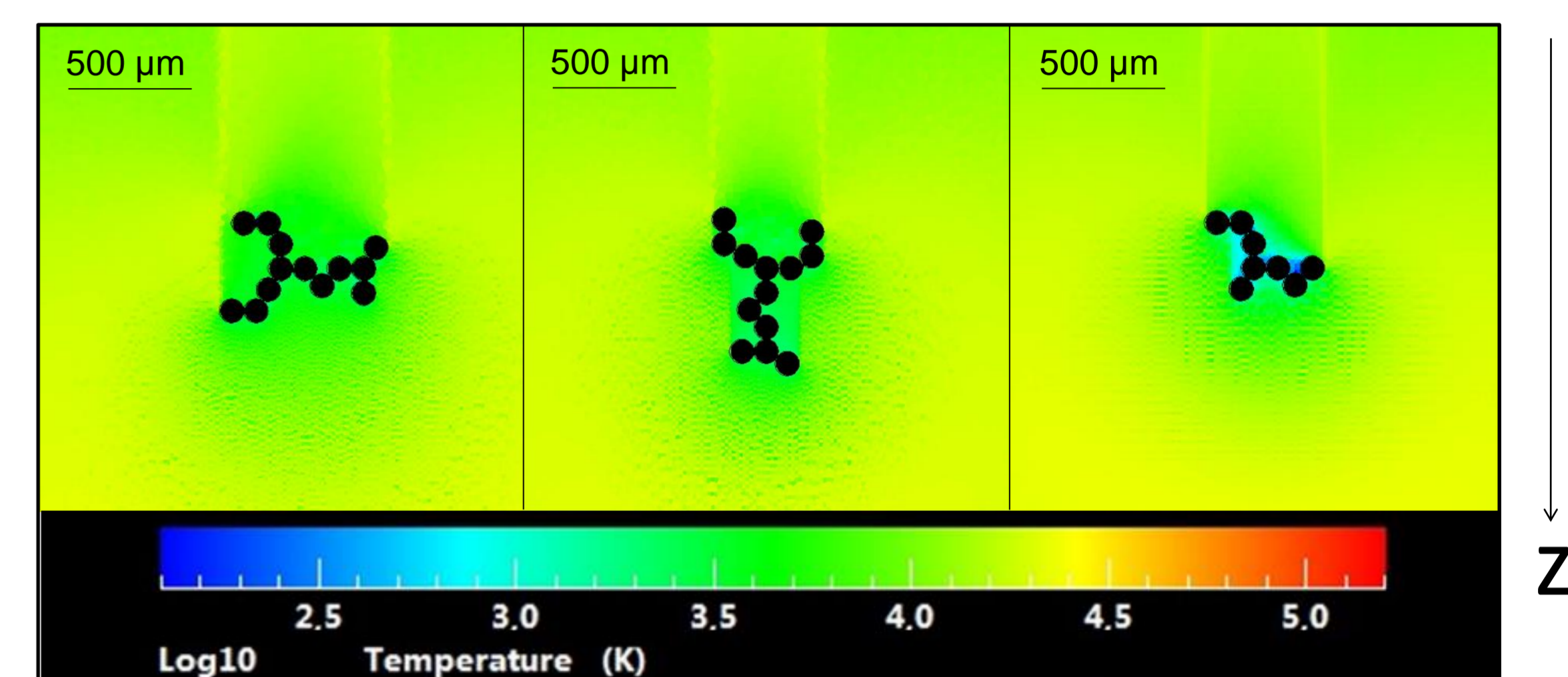
Figure 4: Comparison between the atmospheric entry (at 12 \text{km}\cdot\text{s}^{-1} ) of two fractal aggregates of 13 grains, with orientations at 90^\circ from one another, and a fractal aggregate of 8 grains.
