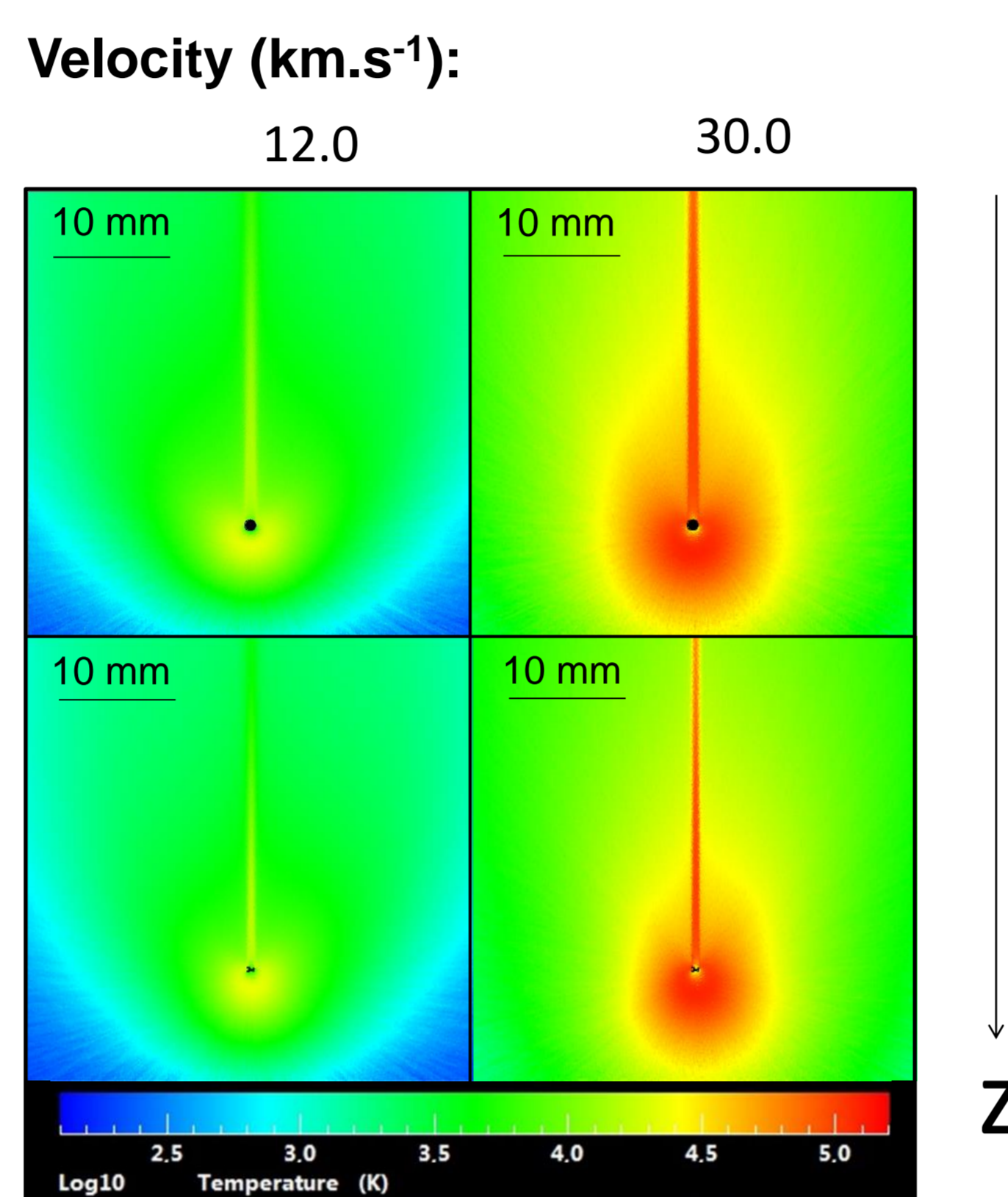
Figure 2: Comparison between atmospheric entry of a 1 mm diameter sphere and a fractal aggregate of 13 grains of 0.05 mm each (large field of view).
