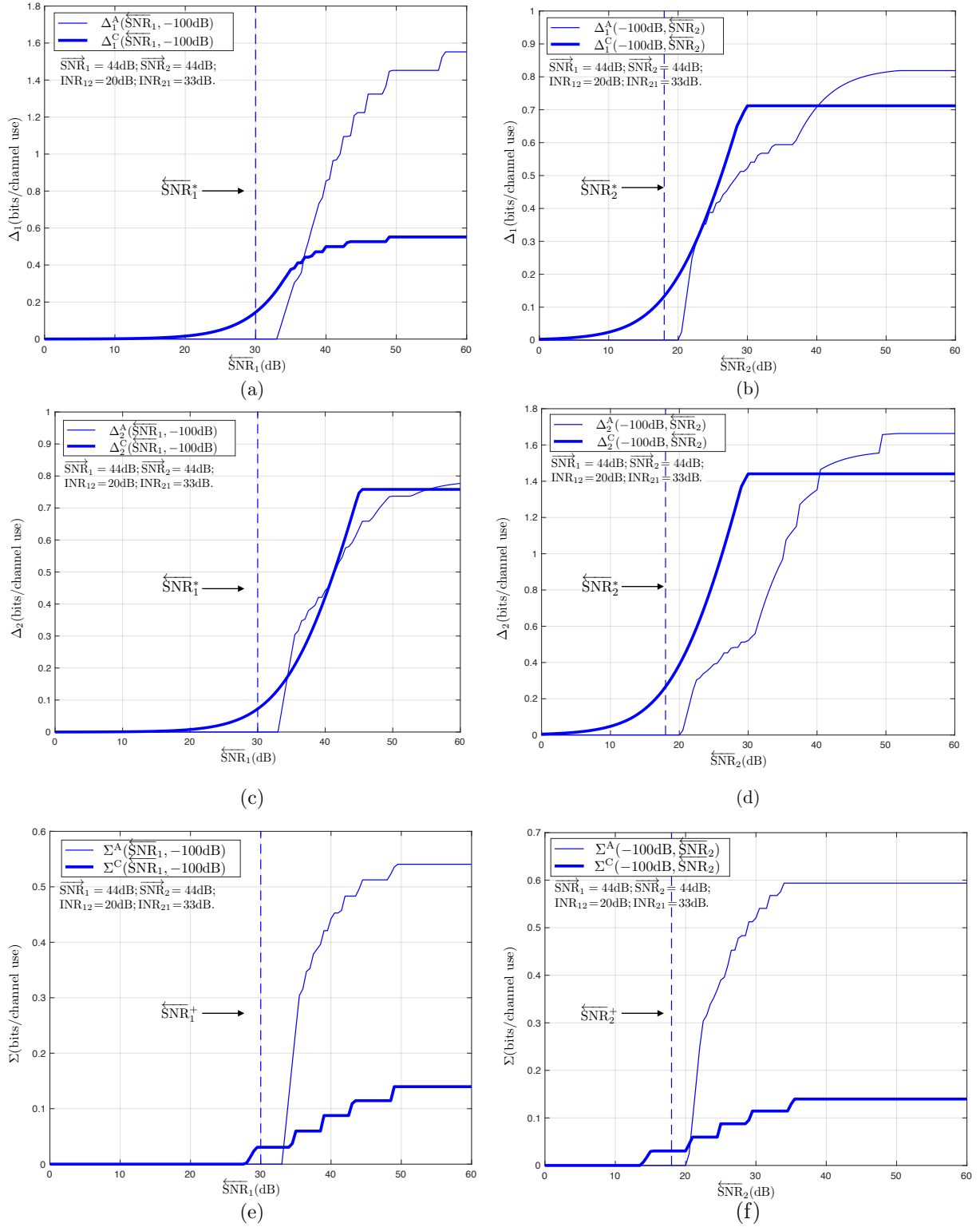
Fig. 6. Improvement metrics \Delta_i^A , \Delta_i^C , \Sigma^A , and \Sigma^C as functions of \overleftarrow{\text{SNR}}_1 and \overleftarrow{\text{SNR}}_2 , with i \in \{1, 2\} , for Example 4.
