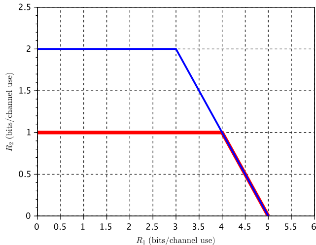
Fig. 5. Capacity regions \mathcal{C}(0,0) (thick red line) and \mathcal{C}(4,0) (thin blue line), with \vec{n}_{11} = 5 , \vec{n}_{22} = 1 , n_{12} = 3 , n_{21} = 4 .
