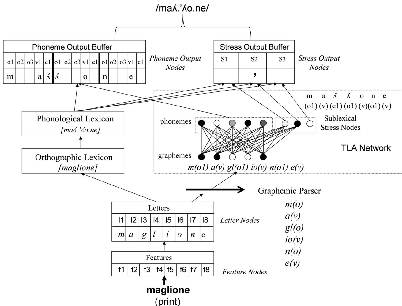
Figure 1. CDP++-Italian. Note f = feature, l = letter, S = Stress, o = onset, v = vowel, c = coda. Numbers correspond to the overall slot number with the letter and feature nodes or the particular slot within an onset, vowel, or coda grouping for the rest of the representations. The thick divisors in the Phoneme Output Buffer represent syllable boundaries. The grapheme and phoneme nodes in the TLN network are simply used as an example, and do not correspond to the actual set of graphemes used in the network. doi:10.1371/journal.pone.0094291.g001
