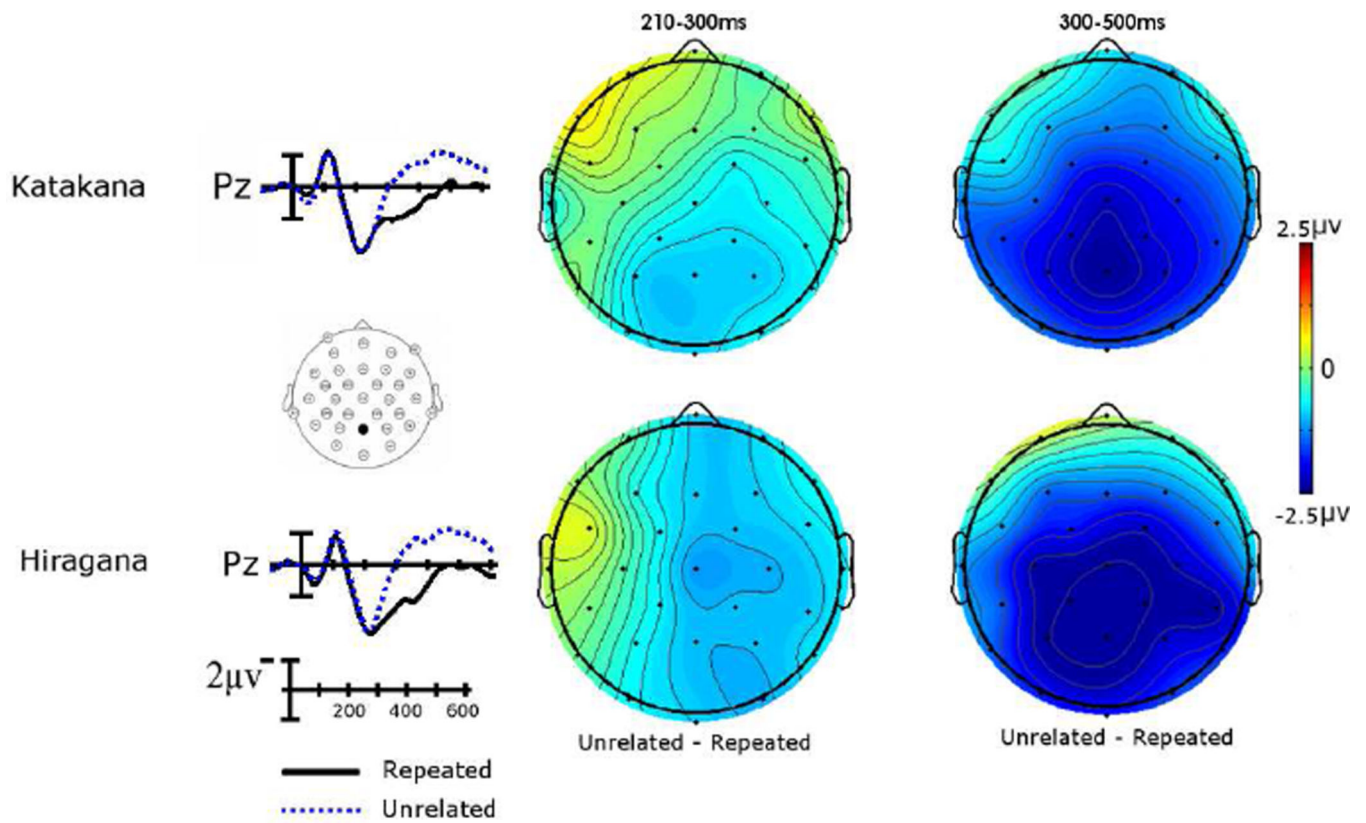
Figure 5. ERP Repetition effects in two epochs 210–300ms and 300–500ms (N400) component for all Katakana prime (upper panels) and Hiragana prime (lower panels) condition. ERPs plotted on the left are from repeated (solid black line) and unrelated (dotted blue line) targets at the Pz site. The voltage maps on the right are from all scalp sites based on average activity of unrelated minus repeated target ERPs averaged across 300–500ms.
