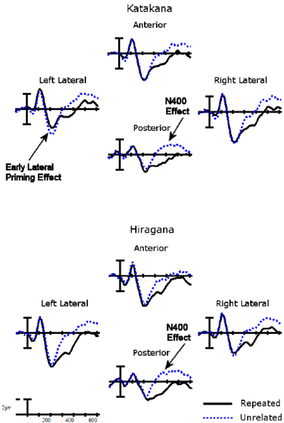
Figure 3. ERPs from all repeated (solid black line) and unrelated (dotted blue line) targets in the Katakana condition (top panel) and the Hiragana condition (bottom panel) at 4 ROIs. Each ROI included 4 electrodes: Anterior ROI included electrode sites FPz, FP1, FP2, FZ, Posterior ROI included sites Pz, O1, O2, Oz, Left Lateral ROI included sites FC5, T3, C3, CP5, and Right Lateral ROI included sites FC6, C4, T4, CP6.
