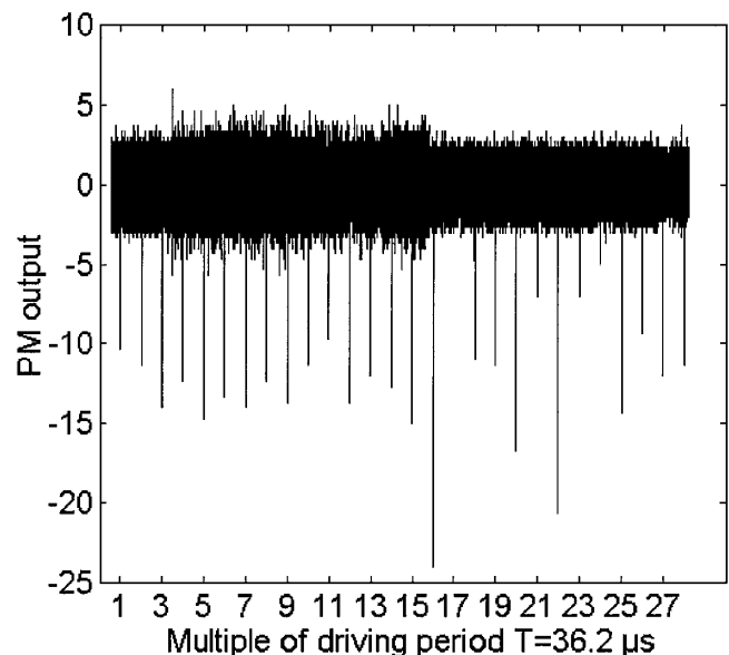
FIG. 4. Flash of light measured by the photomultiplier when a pulse of pressure is applied at the end of the collapse. The acoustic pulse is sent 21.3 \mu\text{s} before the boosted flash at t = 16 T so that it arrives on the bubble 400 ns before the end of the collapse at time. A gain of 90% is obtained when this pressure pulse of 0.7 MPa and 400 ns of duration is applied. The gain is very sensitive to this timing.
