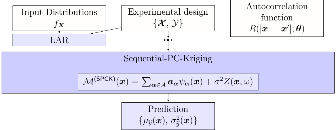
Figure 2: Flowchart for Sequential-PC-Kriging (SPC-Kriging)
