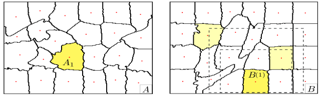
Fig. 7. SPM random search step. The sampling is performed at a decreasing distance around the barycenter of the ANN B(1) of A_1 . The superpixels containing the selected positions (crosses) are the candidates to test.
