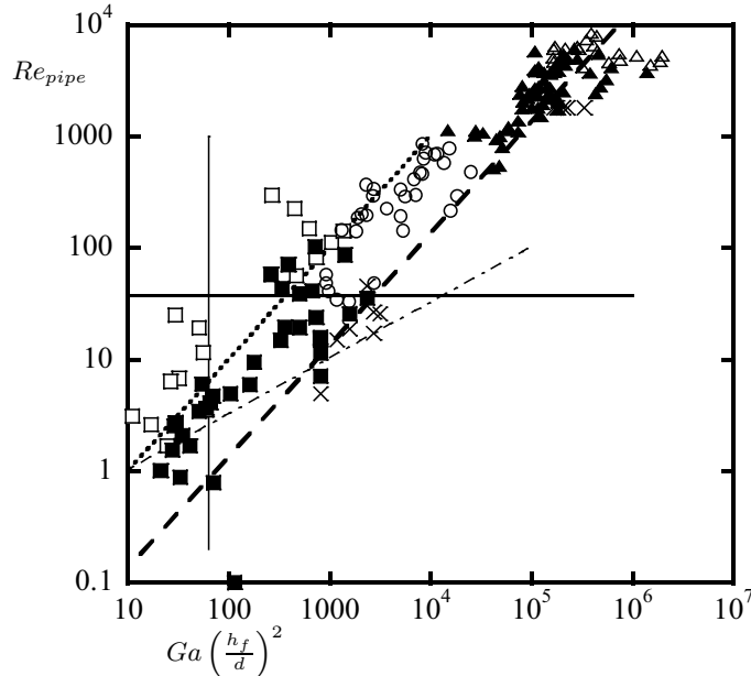
FIGURE 6. Phase-Diagram of the dune patterns in the plane Re_{pipe} , Ga(h_f/d)^2 . The different regimes represented are: ‘no motion’ ( \times ), ‘flat bed in motion’ ( \blacksquare ) and ( \square ) when outside the domain of validity of the model, ‘small dunes’ ( \circ ), ‘vortex dunes’ ( \blacktriangle ), and ‘sinuous dunes’ ( \triangle ). The dashed line is the predicted threshold for particle motion, the horizontal solid line is the predicted instability threshold, and the dotted line indicates the domain of validity of the particle flux law. The dashed-dotted line is the prediction for instability threshold of Charru & Mouilleron-Arnauld (2002) and the vertical solid line is that of Charru & Hinch (2006).
