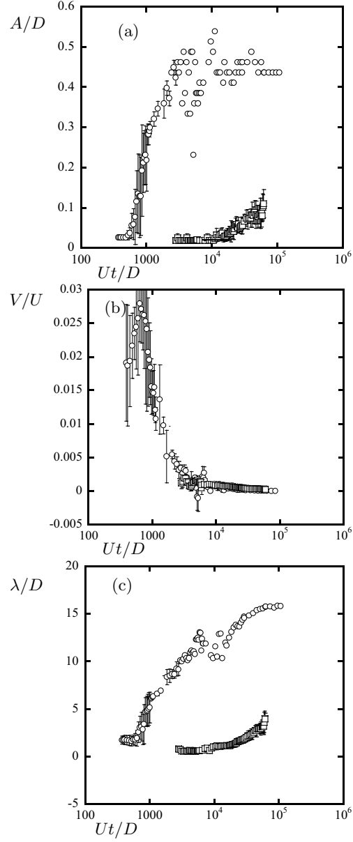
FIGURE 3. Dimensionless dune (a) amplitude, A , (b) velocity, V , and (c) wavelength, \lambda , for batch C in fluid 1 with Q_{pipe} = 3.96 \cdot 10^{-5} \text{m}^3 \cdot \text{s}^{-1} (○, vortex dune regime) and for batch A in fluid 4 with Q_{pipe} = 3.46 \cdot 10^{-5} \text{m}^3 \cdot \text{s}^{-1} (□, small dune regime)
