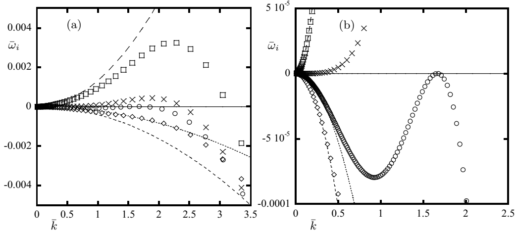
FIGURE 5. (a) Numerical \bar{\omega}_i as a function of \bar{k} for Re_{2D} = 35 ( \diamond ), Re_{2D} = 49.3 ( \circ ), Re_{2D} = 54.3 ( \times ), and Re_{2D} = 70 ( \square ). The lines represent equation (3.15) for Re_{2D} = 35 (small-dashed line), Re_{2D} = 49.3 (dotted line), Re_{2D} = 54.3 (solid line), and Re_{2D} = 70 (long-dashed line) and (b) blow-up.
