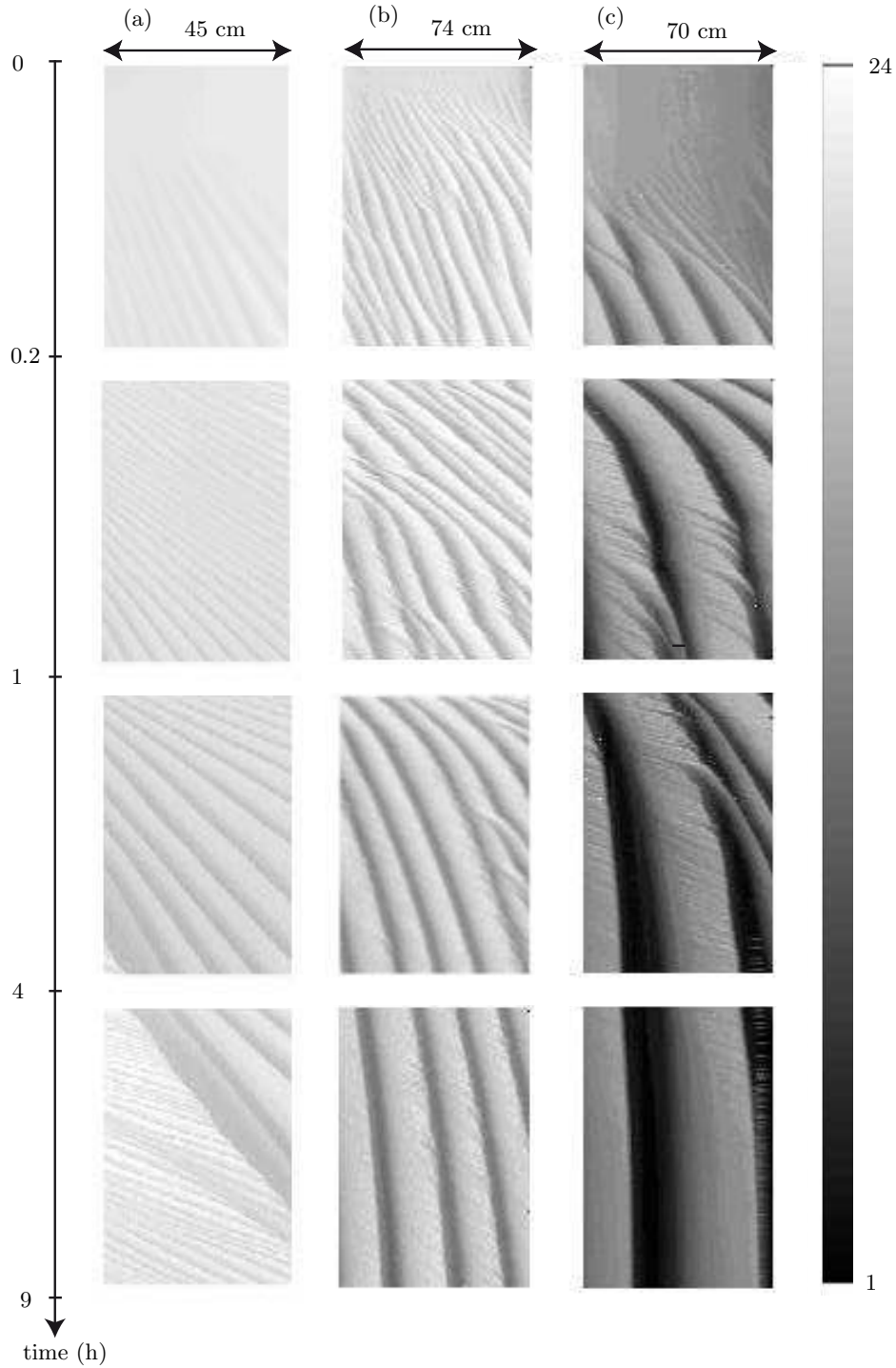
FIGURE 2. Spatio-temporal plots for (a) batch A in fluid 2 with Q_{pipe} = 3.40 \cdot 10^{-5} \text{m}^3 \text{s}^{-1} and h_p^{start} = 22 \text{ mm} (small dune regime), (b) batch A in fluid 1 with Q_{pipe} = 3.79 \cdot 10^{-5} \text{s}^{-1} and h_p^{start} = 21 \text{ mm} (vortex dune regime), and (c) batch C in fluid 1 with Q_{pipe} = 3.96 \cdot 10^{-5} \text{m}^3 \text{s}^{-1} and h_p^{start} = 15 \text{ mm} (vortex dune regime). The grey scale represents the height h_p of the bed in mm.
