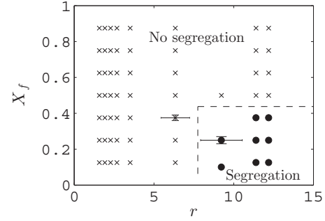
FIG. 9. Phase diagram of the two regimes of segregation observed (x: no segregation and ●: segregation) in the ( X_f, r ) plane for the cylindrical silo with D = 20 \text{ mm} . The dashed lines are indicative of the transition.
