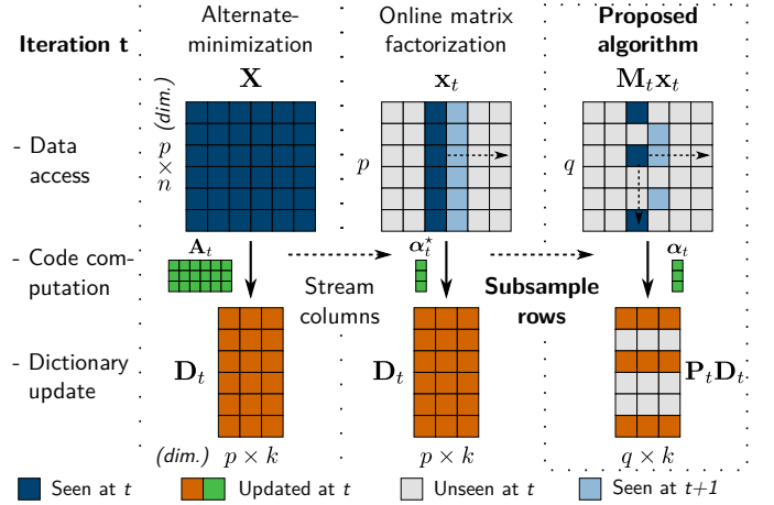
Fig. 1. Stochastic subsampling further improves online matrix factorization to handle datasets with large number of columns and rows. \mathbf{X} is the input p \times n matrix, \mathbf{D}_t and \mathbf{A}_t are respectively the dictionary and code at time t .
