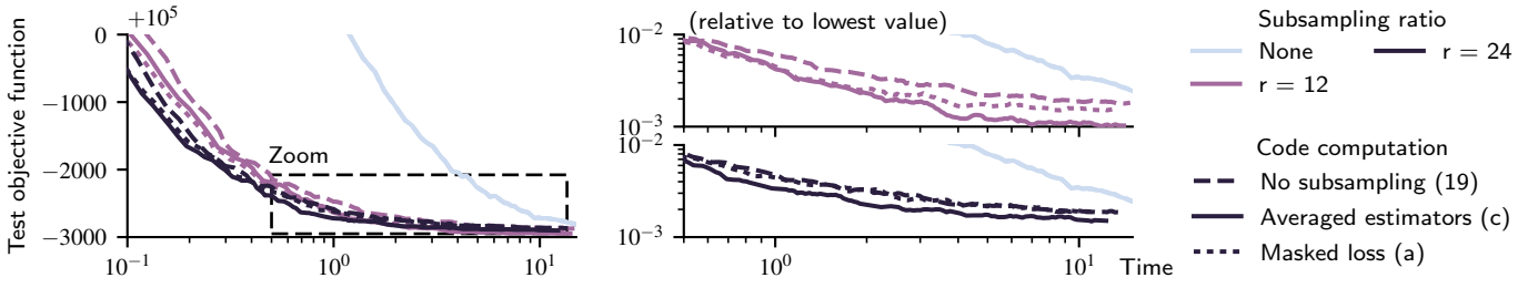
Fig. 6. Approximating code computation with the proposed subsampling method further accelerates the convergence of SOMF. Refining code computation using past iterations (averaged estimates) performs better than simply performing a subsampled linear regression as in [26]
