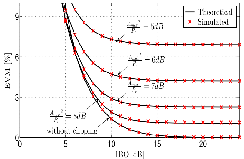
Fig. 5 Theoretical and simulated EVM without predistortion as a function of the IBO, when clipping is activated or not, using a Rapp modeled PA with L_p = 6
