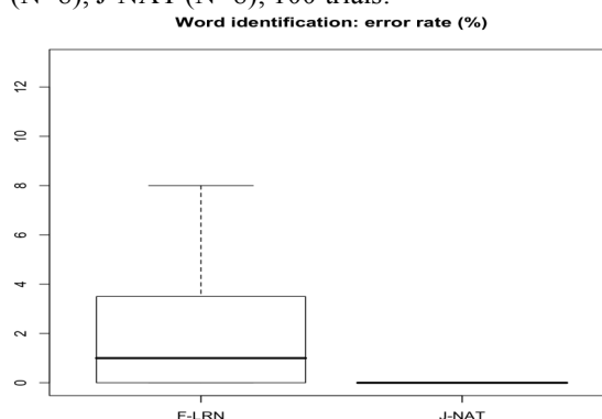
Figure 2: Error rate in word identification: F-LRN (N=8), J-NAT (N=8); 100 trials.
