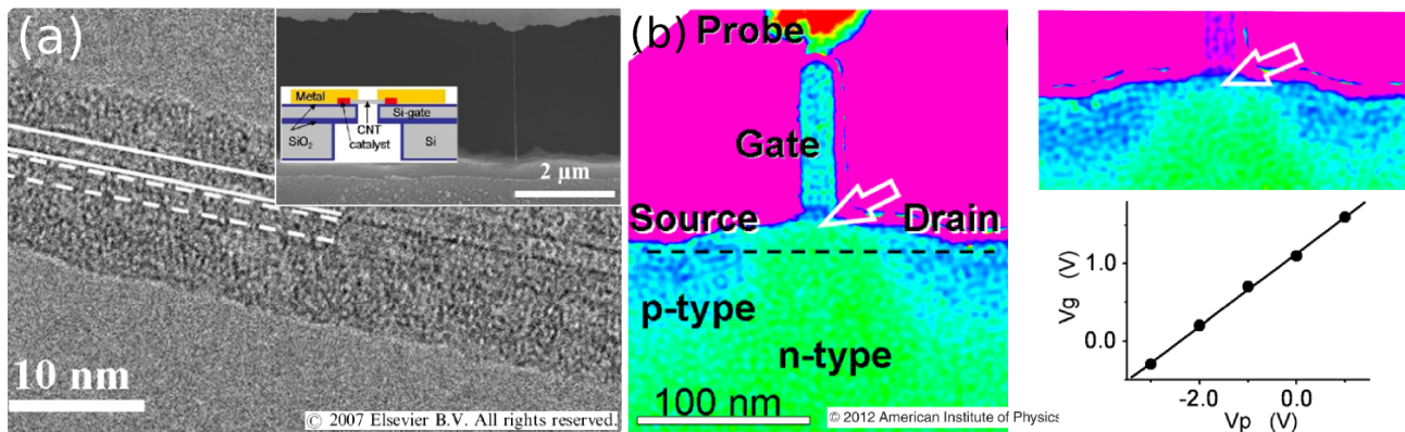
Figure 2: Working devices analyzed in-TEM. a) Field effect transistors (FET) based on CNT bundles mounted in TEM with a multi-contact holder. Observation of CNT during FET function finally showed a huge influence of the electron beam irradiation. Inset is showing a SEM image of the suspended CNT acting as an electron channel (courtesy of (Kim, Kim, et al., 2008)) b) MOSFET electric potential analysis using a moving probe sample holder. Electron holography is used to reveal the electric potential within the MOSFET channel at 0 (left image) and 2 V (right zoomed image). As electron irradiation is perturbing the work of the device (a positive gate tension ( V_g ) is found for a 0 V ( V_p ) probing), the authors have taken into account its influence to get quantitative measurement of the gate work-function. (courtesy of (Ikarashi et al., 2012))
