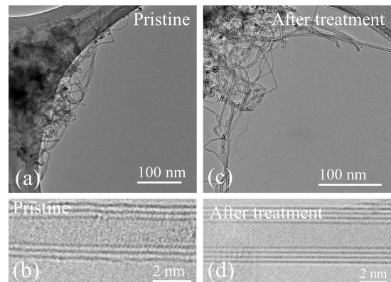
Figure 1. Structural comparison between pristine (a), (b) and doped CNTs (c), (d) at different magnification.
