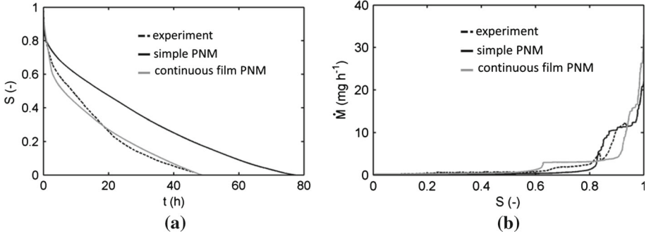
Fig. 16 Comparison between numerical pore network simulations, using the simple PNM and the continuous film PNM, and the experimental result with the \text{SiO}_2 etched network: drying curves (a) and drying rates (b) as reported in Vorhauer et al. (2014)
