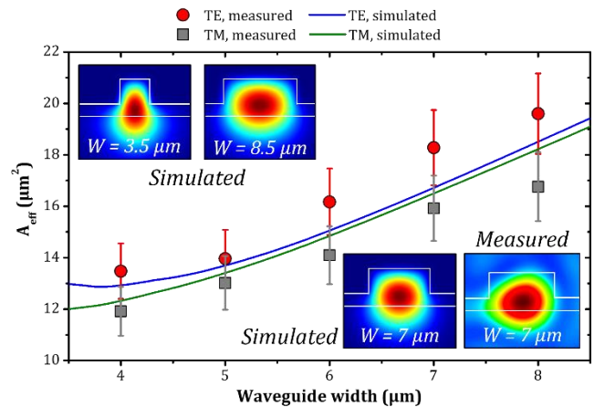
Fig. 4. Comparison between the measured (dotted and squared data) and simulated (solid lines) modal effective area of the quasi-TE mode (red dots and blue line) and the quasi-TM mode (grey squares and green line) as a function of the waveguide width for an operating wavelength of \lambda = 4.6 \mu\text{m} . Right-bottom insets display a modal comparison between the simulated (left) and measured (right) quasi-TE mode profiles of the 7 \mu\text{m} wide waveguide. Inset images at the upper-left hand side show the simulated quasi-TE near-field mode profile of a 3.5 \mu\text{m} (left) and a 8.5 \mu\text{m} (right) wide waveguide.
