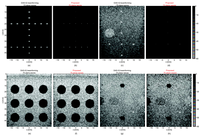
Fig. 4. Comparison of the proposed BF method ((b), (d), (f), (h)) with DAS BF ((a), (c), (e), (g)) for all challenge datasets, using 75 plane-waves.
