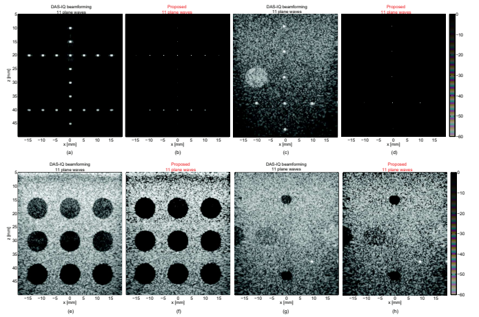
Fig. 3. Comparison of the proposed BF method ((b), (d), (f), (h)) with DAS BF ((a), (c), (e), (g)) for all challenge datasets, using 11 plane-waves.
