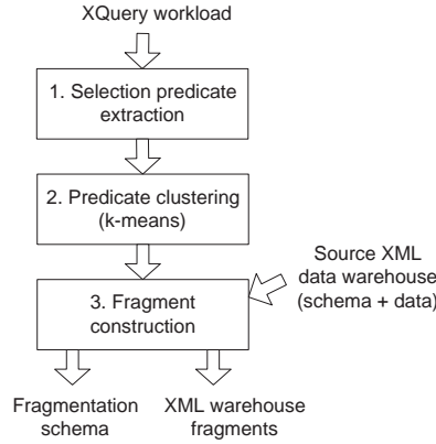
Figure 5 K -Means-Based XML Data Warehouse Fragmentation Overview
