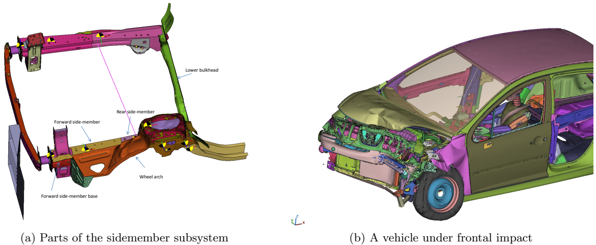
Figure 10: Sidemember subsystem
