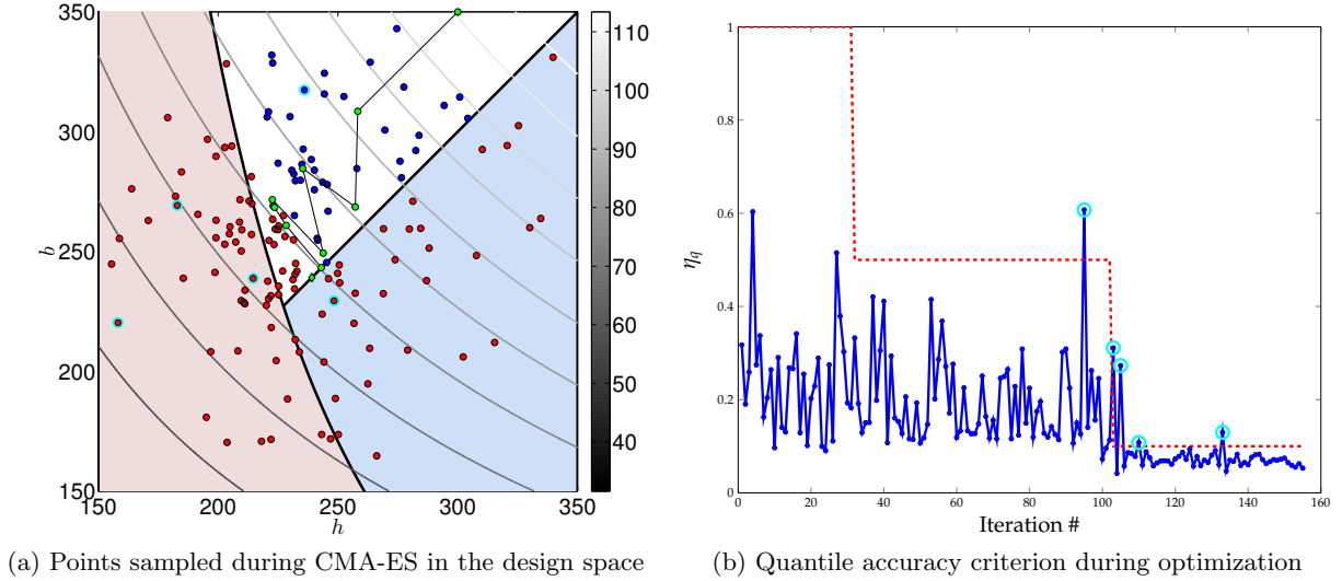
Figure 5: Convergence of the column under compression problem. The left panel shows the evolution of CMA-ES in the design space. The blue and red dots fall respectively in the feasible and unfeasible sets. The green ones are the successive best sample points. In the right panel, the evolution of the local accuracy criterion is shown with respect to the number of iterations. In the two figures, the points corresponding to enrichment have been circled in cyan.
