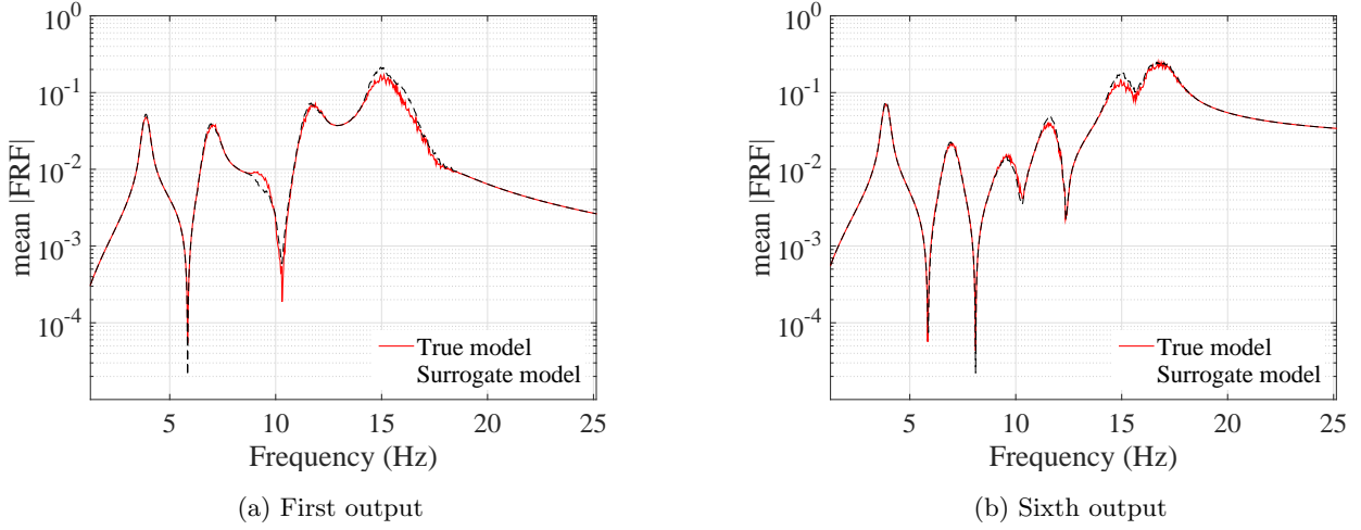
Figure 24: Mean of the FRF of the 6-DOF system at 2 outputs, evaluated at 10,000 MC sample points by the true model (red line) and the surrogate model (black line).
