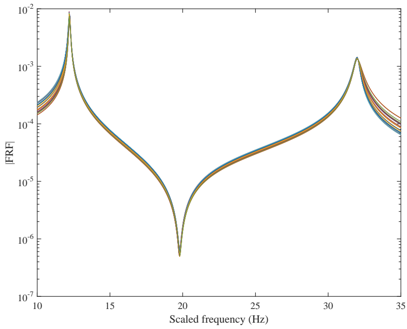
(b) FRFs after frequency transformation.
