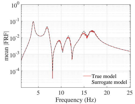
Figure 30: Mean of the FRF of the 6-DOF system at 4 outputs, evaluated at 10,000 MC sample points by the true model (red line) and the surrogate model (black line).
