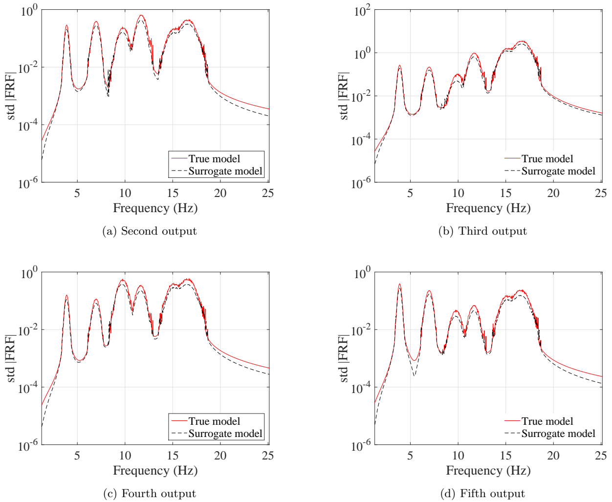
Figure 31: Standard deviation of the FRF of the 6-DOF system at 4 outputs, evaluated at 10,000 MC sample points by the true model (red line) and the surrogate model (black line).
