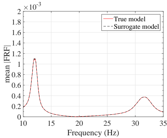
(c) The proposed method in this work. Sparse PCEs with order less than 8 and stochastic frequency transformation
