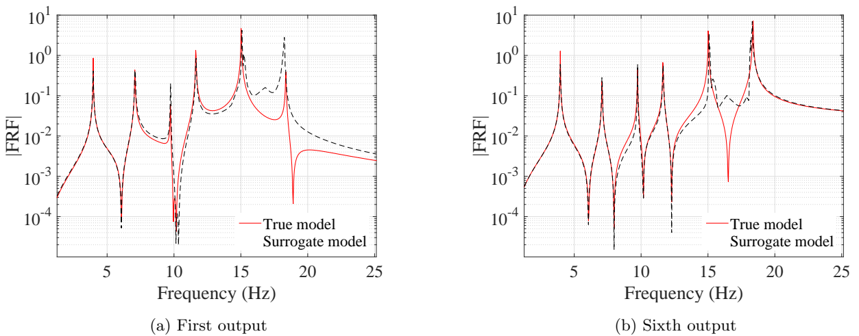
Figure 23: The worst FRFs (out of 10,000) predicted by the surrogate model at 2 outputs, evaluated by the true model (red line) and the surrogate model (black line).
