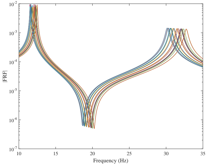
(a) FRFs before frequency transformation.
