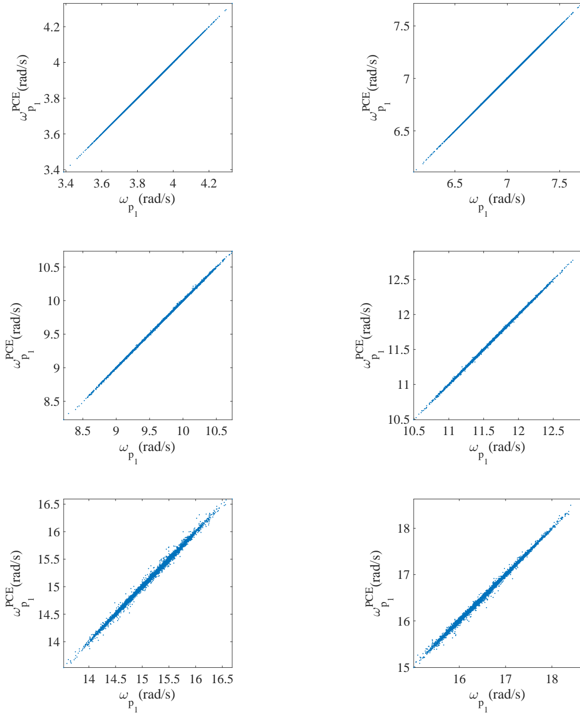
Figure 20: The eigenfrequencies predicted by the surrogate model versus obtained by the true model, evaluated at 10,000 MC samples.
