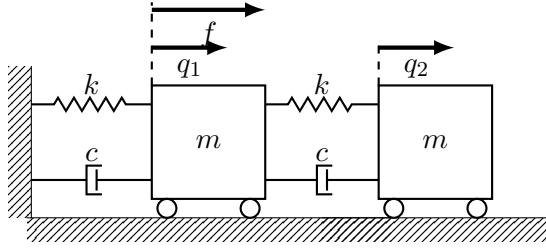
Figure 4: 2-DOF system
