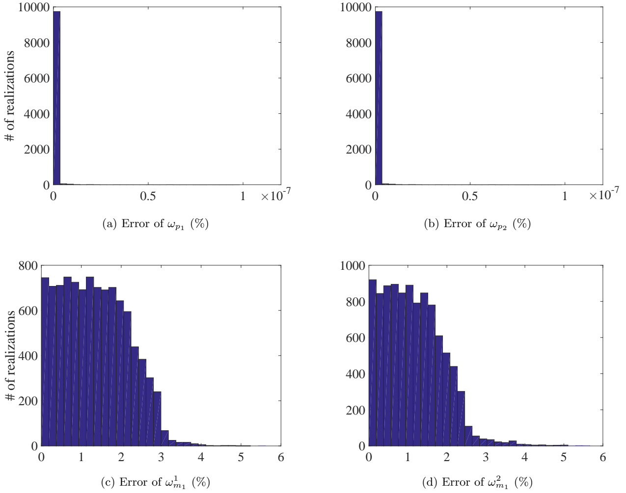
Figure 8: Error of the selected frequencies predicted by PCE surrogate model, evaluated by Eq. (24).
