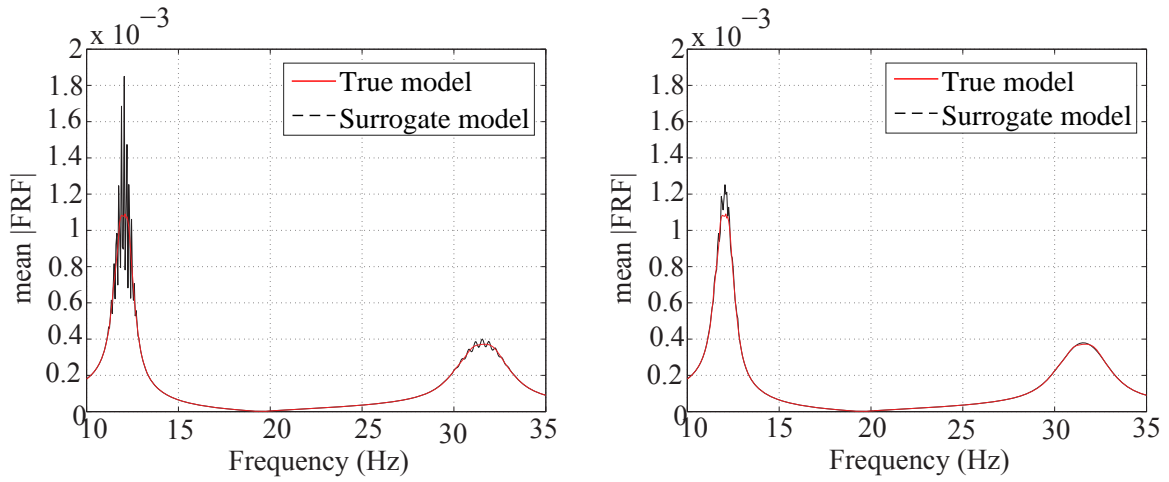
(a) Direct use of PCE with order 50. Shown in Jacquelin et al. (2015a,b) (b) PCE with order 50 and Aitken's transformation. Proposed in Jacquelin et al. (2015b)
