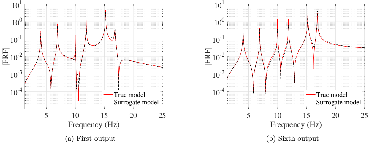
Figure 22: Typical FRFs predicted by the surrogate model at 2 outputs, evaluated by the true model (red line) and the surrogate model (black line).
