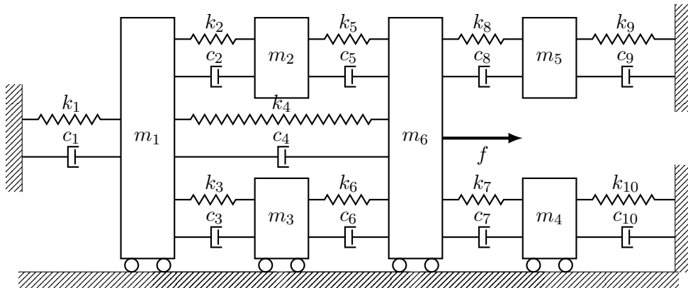
Figure 17: The 6-DOF system
