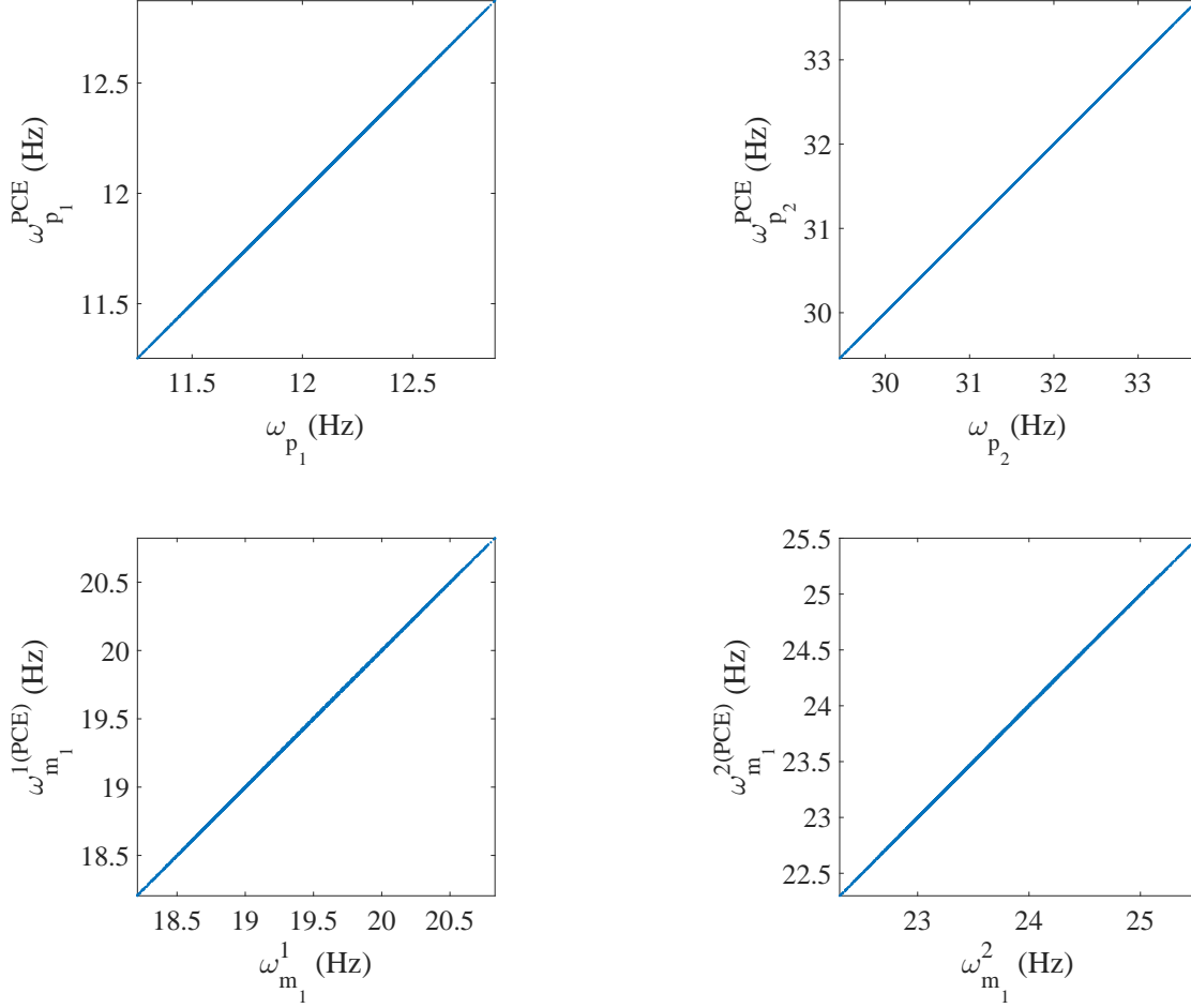
Figure 7: Selected frequencies predicted by the surrogate model versus by the true model. upper row: eigenfrequencies, lower row: frequencies where minimum amplitude occurs, see matrix (16) for notations.
