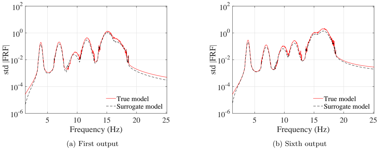
Figure 25: Standard deviation of the FRF of the 6-DOF system at 2 outputs, evaluated at 10,000 MC sample points by the true model (red line) and the surrogate model (black line).
