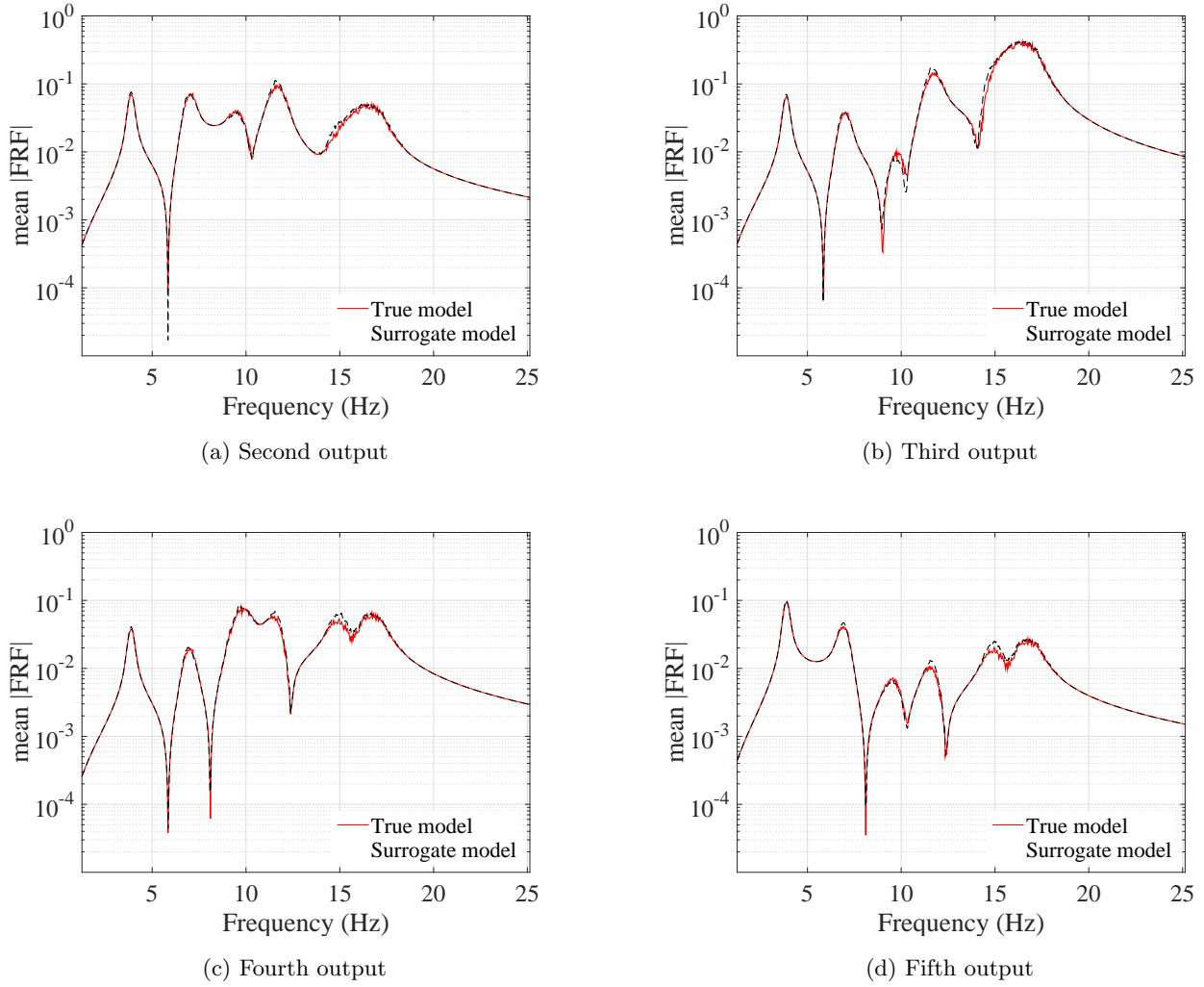
Figure 30: Mean of the FRF of the 6-DOF system at 4 outputs, evaluated at 10,000 MC sample points by the true model (red line) and the surrogate model (black line).
