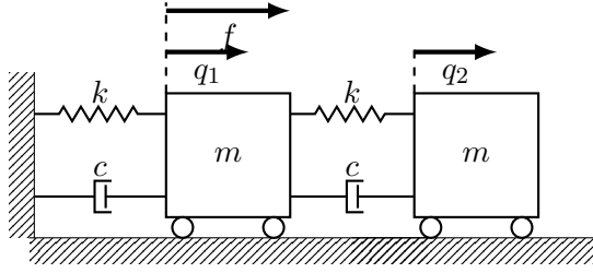
Figure 4: 2-DOF system
