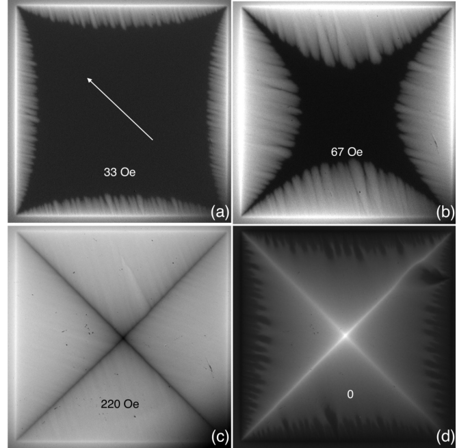
FIG. 3. Same as Fig. 1 in the presence of the in-plane field H_{\parallel} = 965 Oe along one of the diagonals of the square. T = 6 K. Values of H_{\perp} are shown on the pictures. Arrow shows the direction of H_{\parallel} .
