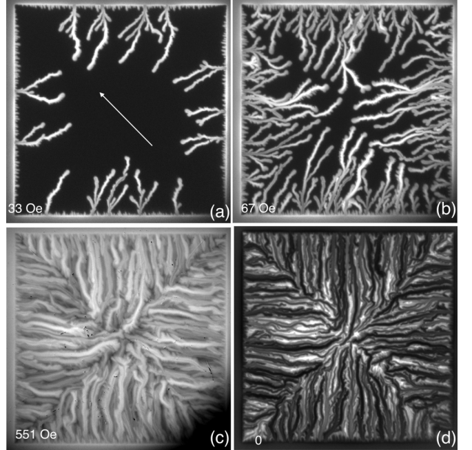
FIG. 6. TMA patterns at T = 3.2 K in the presence of H_{||} = 965 Oe along one of the diagonals of the square. (a–c) Increasing H_{\perp} and (d) trapped flux pattern with negative dendrites. Values of H_{\perp} are shown on the pictures. Arrow shows the direction of H_{||} . Dendrites are generated symmetrically on all square sides but their branches tend to turn across H_{||} .
