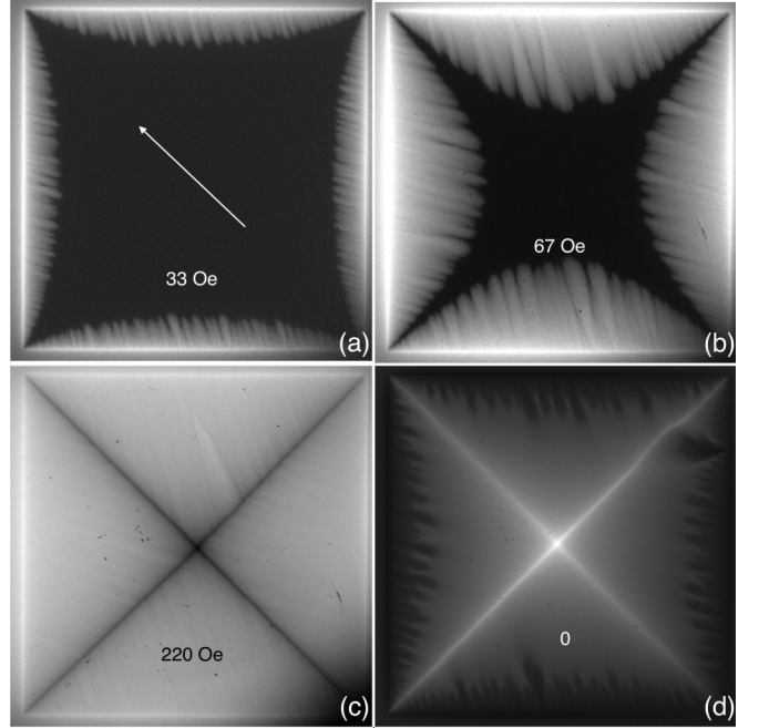
FIG. 3. Same as Fig. 1 in the presence of the in-plane field H_{||} = 965 Oe along one of the diagonals of the square. T = 6 K. Values of H_{\perp} are shown on the pictures. Arrow shows the direction of H_{||} .
