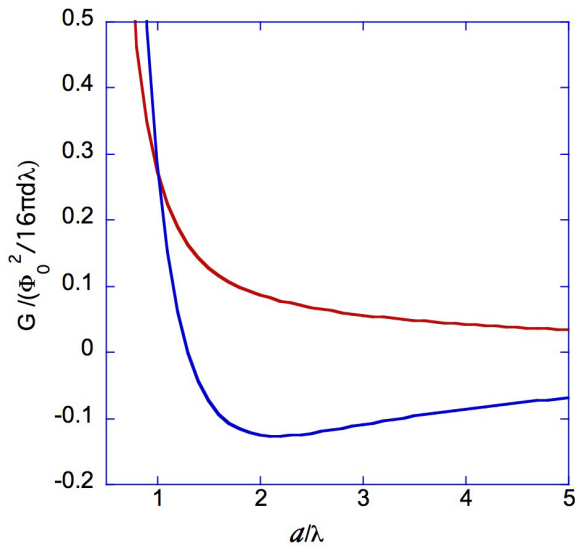
FIG. 9. Gibbs potential G for in-plane vortices as a function of the intervortex distance a for a single vortex row in 100- (top) and 200-nm (bottom curve) films at H_{||} = 1 kOe. See details of the calculations in the text.
