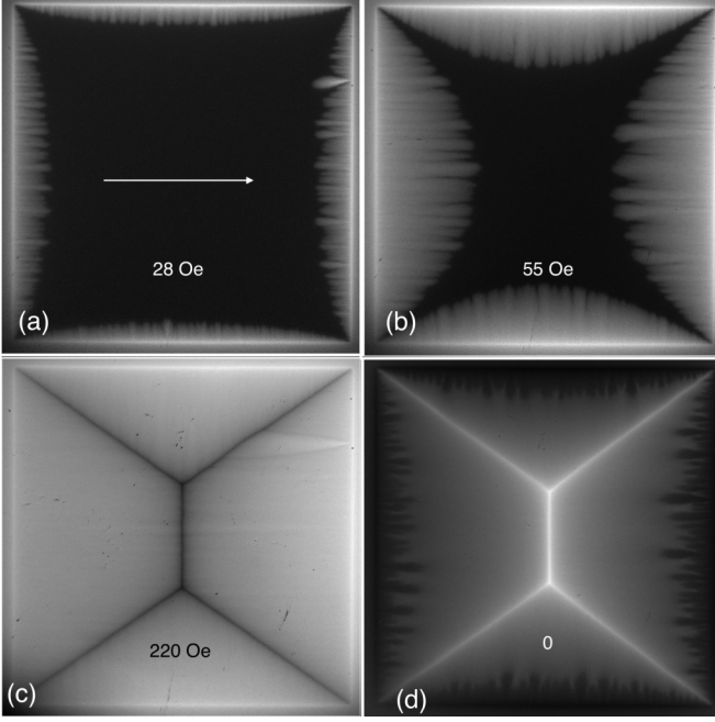
FIG. 2. Same as Fig. 1 in the presence of the in-plane field H_{||} = 965 Oe along the horizontal side of the square. T = 6 K. Values of H_{\perp} are shown on the pictures. Arrow shows the direction of H_{||} .
