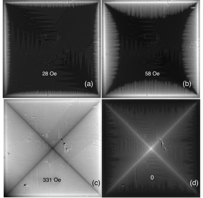
FIG. 1. Normal flux patterns in 2.5 \times 2.5 -mm square sample of 200-nm-thick Nb film at 6 K in the absence of the in-plane field. (a–c) Magneto-optic images in the increasing normal field H_{\perp} ; (d) trapped flux pattern after reducing field to zero from a maximum of 662 Oe. Values of H_{\perp} are shown on the pictures. The brightness of the magneto-optic contrast corresponds to the normal flux density. Zigzag structures across the image in (d) correspond to the in-plane domain walls in the garnet indicator film.
