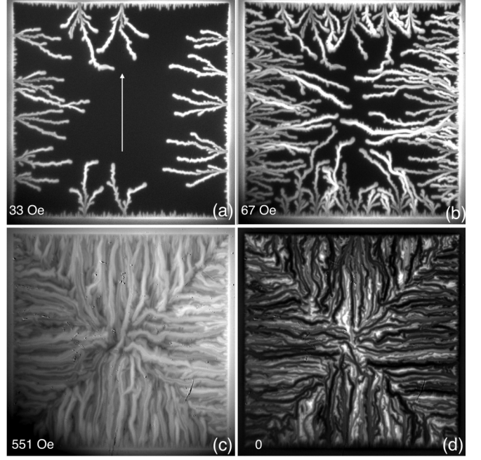
FIG. 5. TMA patterns at T = 3.2 K in the presence of H_{||} = 965 Oe along the vertical side of the square. (a–c) Increasing H_{\perp} and (d) trapped flux pattern showing negative dendrites formed at decreasing H_{\perp} . Values of H_{\perp} are shown on the pictures. Arrow shows the direction of H_{||} . Dendrites are preferentially generated on the square sides parallel to H_{||} and have longer branches across H_{||} .
