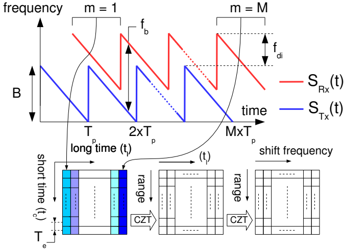
Fig. 2: Instantaneous frequency over M transmitted ramps
