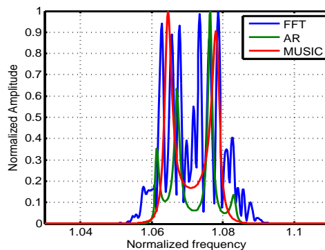
Fig. 5: Simulation of spectra with FFT, AR and MUSIC algorithm
