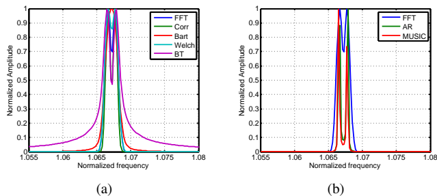
Fig. 4: Simulation of CZT radar spectra (a) Non-Parametric methods ; (b) AR method and MUSIC algorithm.
