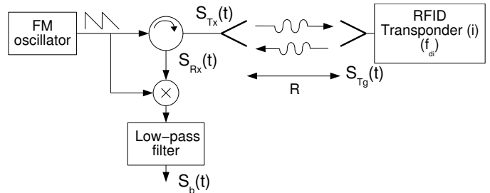
Fig. 1: Setup of FMCW radar based RFID localization system
