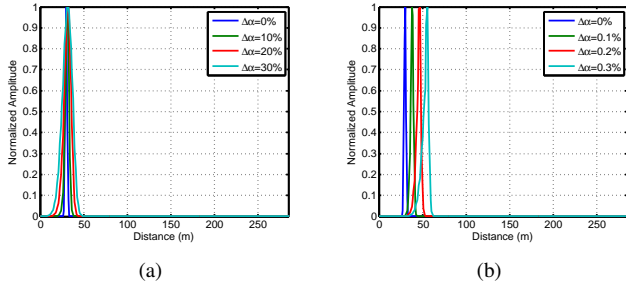
Fig. 6: Effect of sweep non-linearity (a) Case 1: non-linearity at FMCW reader and RFID transponder ; (b) non-linearity at RFID transponder.
