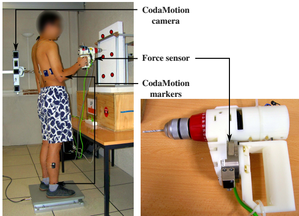
Figure 8: Force and motion capture instrumentation for the drilling activity. A commercial drill has been modified to embed a force sensor. The red circles on the slab represent the drilling points.
