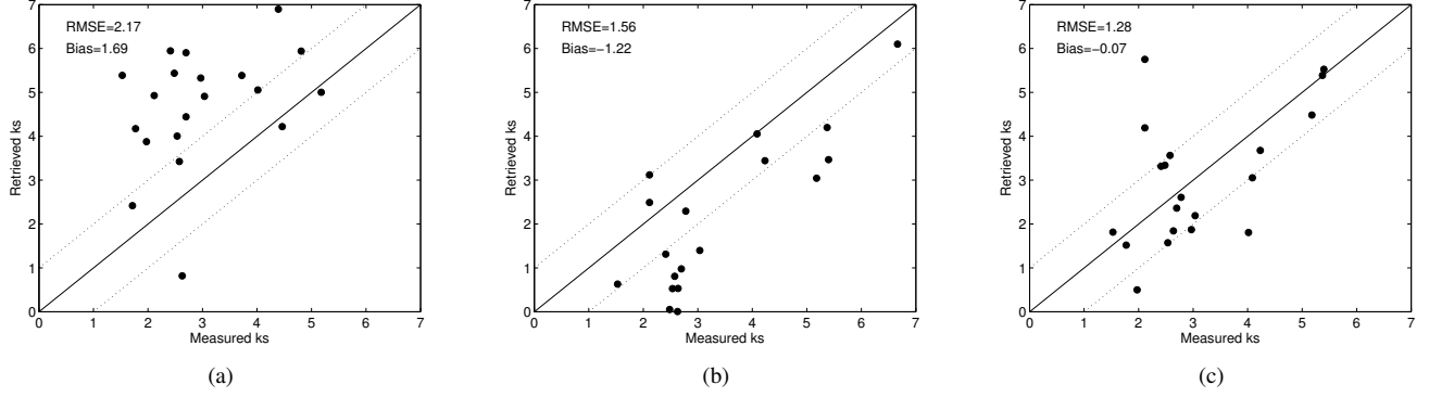
Fig. 14. Comparison between ground in situ measured and retrieved surface roughness using \gamma_{HH} (a) 24^\circ and 31^\circ ; (b) 31^\circ and 43^\circ ; (c) 24^\circ and 43^\circ .
