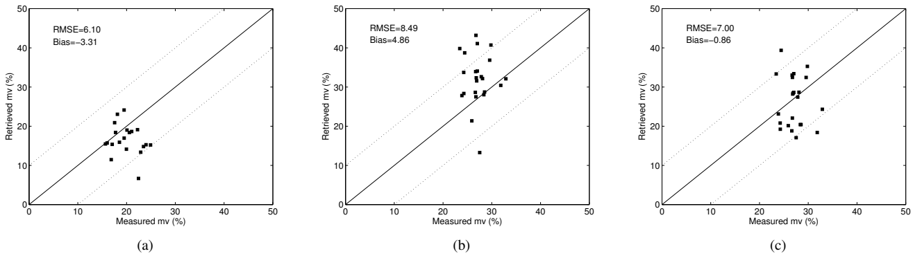
Fig. 15. Comparison between ground in situ measured and retrieved soil moisture (a) 24^\circ (and 31^\circ for roughness); (b) 31^\circ (and 43^\circ for roughness); (c) 24^\circ (and 43^\circ for roughness).
