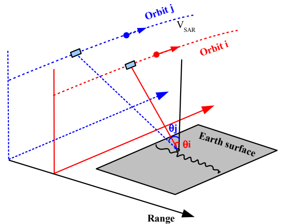
Fig. 6. Multi-angular SAR configuration.
