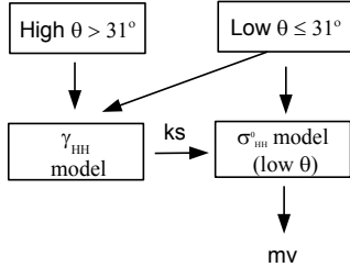
Fig. 13. Multi-angular SAR approach for soil parameter retrievals.
