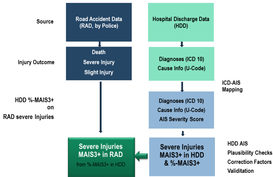
Figure A 6 Data and procedural options in Austria for the calculation of the the of the MAIS \geq 3 indicator
