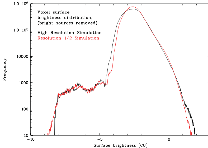
Figure A2. The surface brightness distributions of two Ly \alpha cubes at z = 0.75 after removing the bright sources. The black curve shows the results obtained in the simulation used throughout the paper, whereas the red histogram is derived from a simulation with a spatial and mass resolution of a factor 8 worse, as in Fig. A1. Unlike for the bright sources, there is little difference in the two histograms, indicating – as expected – that for areas of moderate overdensity the simulation has reached convergence. There is a small number of pixels inside filamentary structures that exhibit surface brightnesses of about half a dex higher in the higher resolution cube, but those are so rare and spread out over wide volumes that they do not contribute significantly to the brightness of one specific filament.
