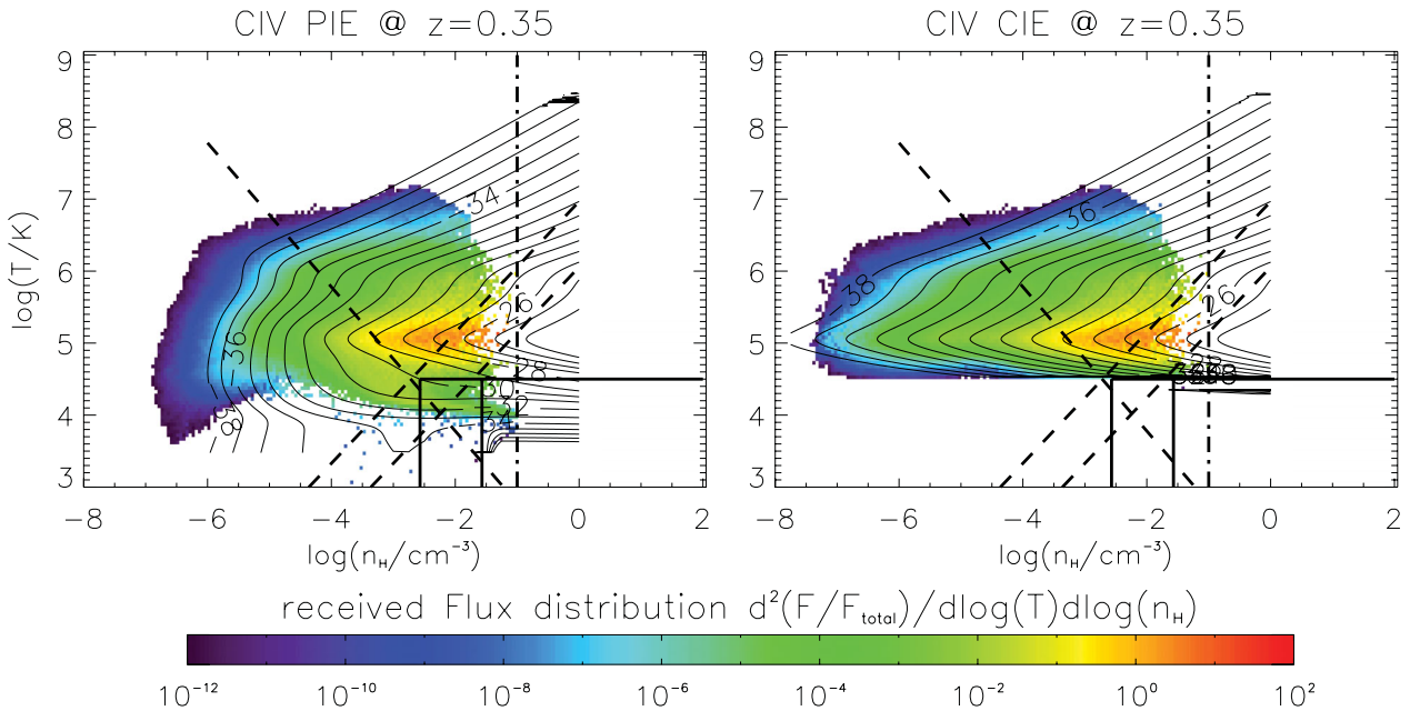
Figure 3. Same structure as in Fig. 1, now showing C IV at a redshift of z = 0.35 .
