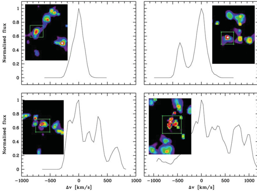
Figure 13. Examples of the four different classes of velocity profiles, here for the O\text{VI} emission. Note that the resolution of the representation chosen here (after resampling to the FIREBall specifics) is about 80\text{ km s}^{-1}\text{ pixel}^{-1} . The coloured insets show the spatial images collapsed along the z -axis as in Fig. 9. The velocity plots are derived by collapsing the area shown in green along the other two axes, and translating the differences in the z direction to velocities (for details see text). The upper left-hand panel shows a single peak in the spatial image, but the z direction yields a profile that can be fitted well by a single Gaussian. The upper right-hand panel is an example of a similarly simply spatially structured source, but with a double-peaked velocity profile. The lower left-hand panel exhibits again a single peak in x - y , but this time a much more complex, multiply peaked velocity profile. The lower right-hand panel, finally, has a complex spatial structure, in combination with a multiply peaked velocity profile. Note the slight change in scale for the velocity plot for this example. Both the C\text{IV} and the \text{Ly}\alpha compact sources show velocity profiles very similar to the ones depicted here, but the interpretation for the \text{Ly}\alpha emission is complicated by a variety of factors (see text for details).
