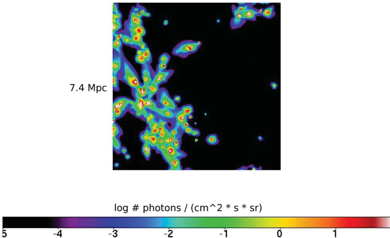
Figure 15. Example of a typical ‘filamentary’ structure in O\text{VI} at z_{\text{em}} = 1.1 . The size of the field is again 900 \times 900 \text{ arcsec}^2 , translating to 7.4 \times 7.4 \text{ Mpc}^2 . The depth ( 5 \text{ \AA} ) represents 5.1 \text{ Mpc} . Note the different scale in brightness as compared to Fig. 14: the filaments connecting the bright sources are now about three orders of magnitude fainter. The physical conditions of the gas forming the filamentary structures are very similar to the ones seen in \text{Ly}\alpha : the metallicity of such gas ranges from 10^{-3.5} up to 10^{-2.5} , which is the main factor in those to be less bright. Note, however, that the flux is concentrated towards the bright sources even more than in the case for \text{Ly}\alpha .
