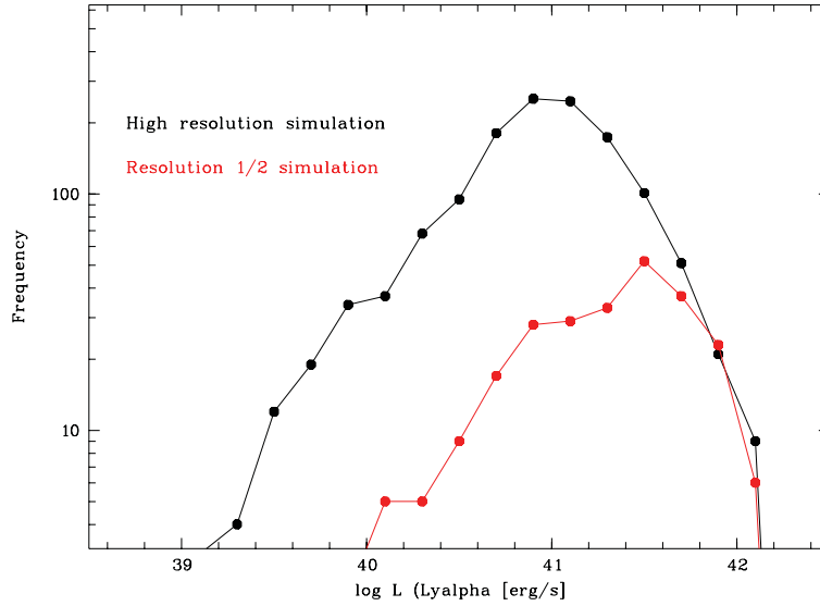
Figure A1. The luminosity distribution of the bright Ly \alpha sources at z = 0.75 extracted with the same source finding parameters in two cubes of the same volume but with different spatial and mass resolutions. The black curve shows the results obtained in the simulation used throughout this paper, whereas the red histogram is derived from a simulation with a spatial resolution of a factor of 2 lower (in each dimension), and hence a mass resolution of a factor of 8 worse. Note the strong dependence of the number of sources on the resolution: increasing the resolution in this fashion leads to about five times more sources in the same volume. The majority of the new sources, however, are much less luminous, and hence their contribution to the total light is small. The two curves start matching around \log L \sim 41.6 , and hence we conclude that down to this luminosity the simulation has converged.
