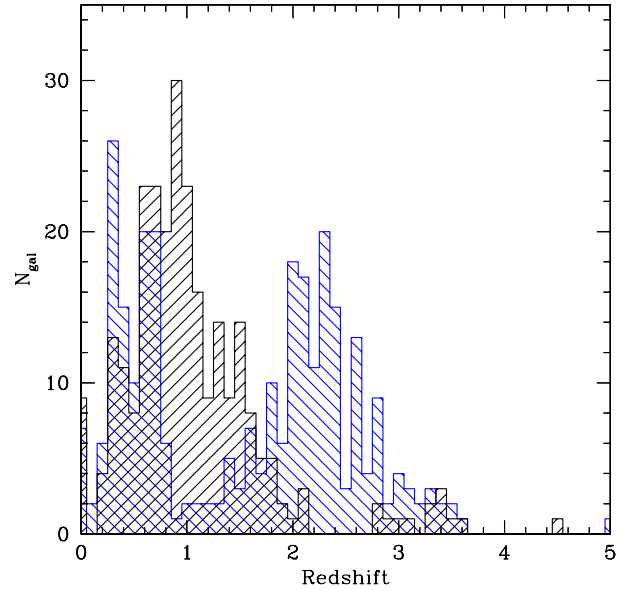
Fig. 17. Redshift distribution of galaxies with the most reliable redshifts (flags 3 and 4), from the LRBLUE setup (hatched blue histogram), and from the LRRED setup (hatched black histogram).
