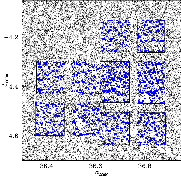
Fig. 6. Distribution in (\alpha, \delta) of galaxies observed in the Ultra-Deep 23 \leq i_{AB} \leq 24.75 sample (heavy symbols) over the photometric parent sample (dots).
