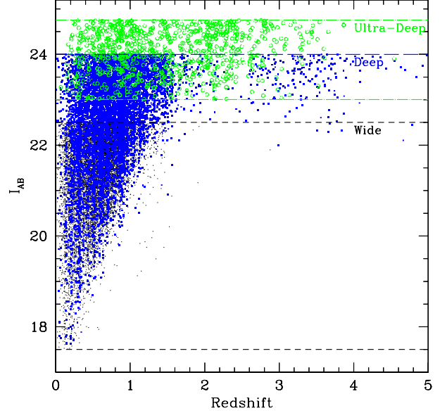
Fig. 19. Distribution of apparent I_{AB} apparent magnitudes for the VVDS-Wide (dots), VVDS-Deep (squares), and Ultra-Deep (open circles) samples.
