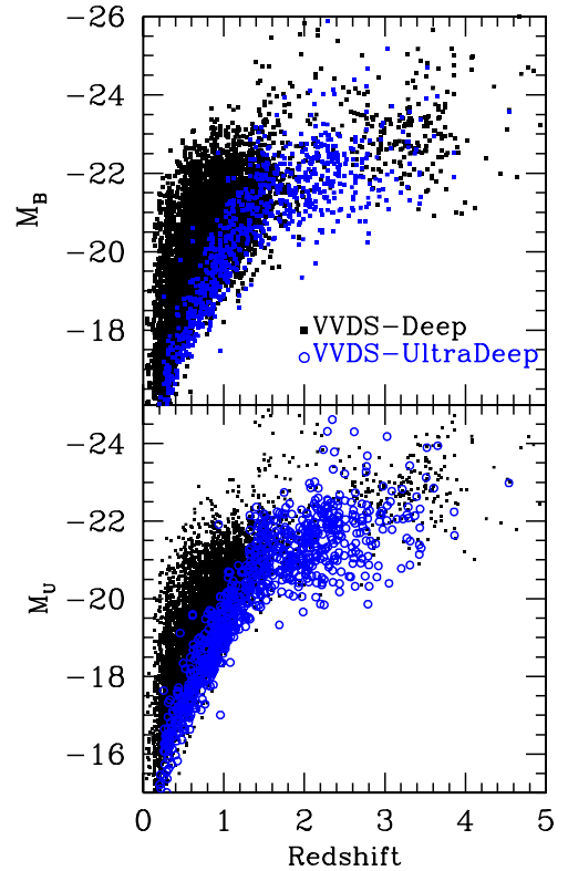
Fig. 20. Distribution of B -band (top) and u -band (bottom) absolute magnitudes for the VVDS-Deep (dots), and Ultra-Deep (open circles) samples.
