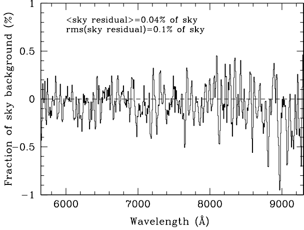
Fig. 2. Sky background-subtraction accuracy expressed as the ratio of the sky-subtracted spectrum over the observed sky spectrum, obtained from the 18 h stack of VIMOS-LRRED observations for the VVDS-Ultra-Deep survey.
