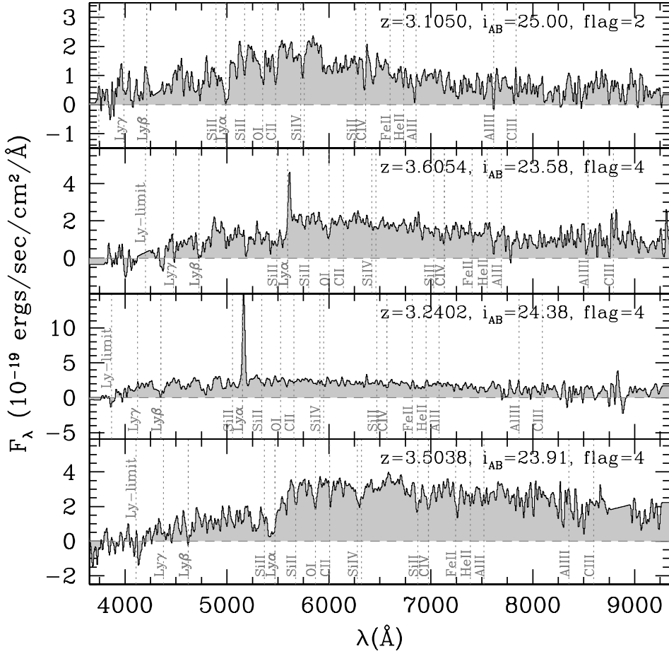
sample VUDS spectra with 3 < z < 4
