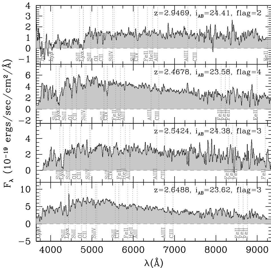
sample VUDS spectra with 2 < z < 3
