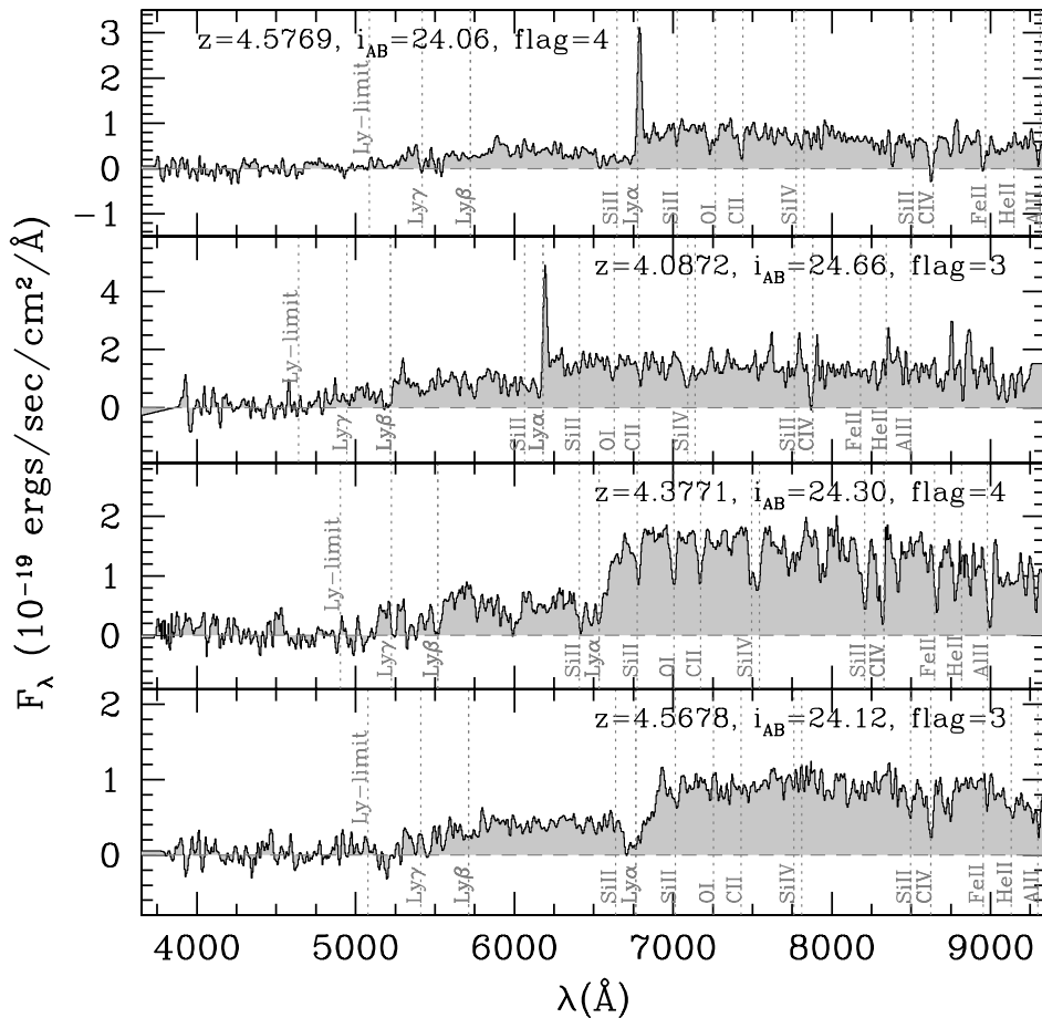
sample VUDS spectra with 4 < z < 5
