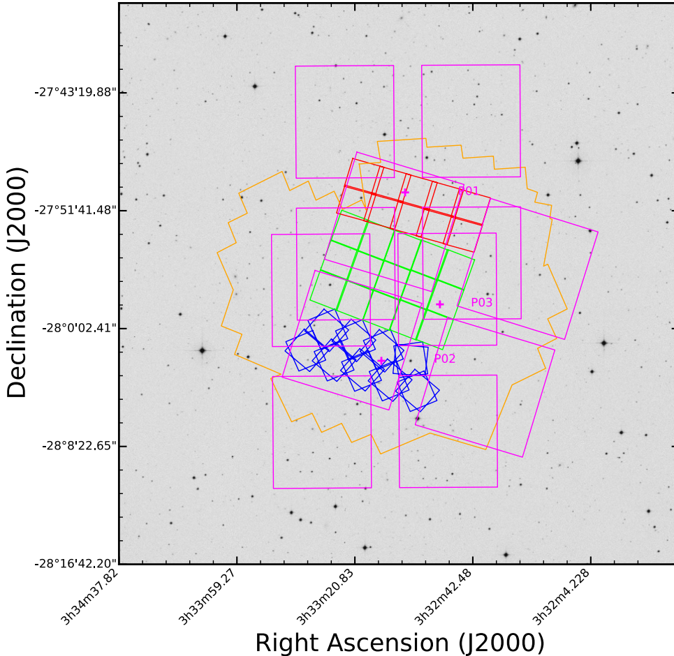
Fig. 2. Layout of the observed 3 VUDS VIMOS pointings in the ECDFS field. The centre of each VIMOS pointing is identified by a cross with the pointing number (see Table 3), while the imprint of the 4 quadrants is plotted in magenta. The positions of the CANDELS WFC3 deep area is indicated in green, the CANDELS wide area in blue. The red region indicates the WFC3 coverage of the ERS. The outline of the existing ACS- F814W imaging is identified in orange. The size of the image is 0.67 \times 0.67 \text{ deg}^2 .
