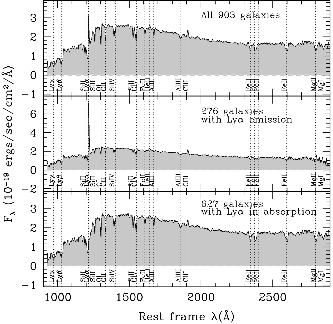
Fig. 19. Average rest-frame spectra ( F_\lambda ) of galaxies with flags 3 and 4 in VUDS with 2 \leq z \leq 3 : top : stack of all galaxy spectra; middle : stack of galaxies with Ly- \alpha in emission; bottom : stack of galaxies with Ly- \alpha in absorption (this stack is from a subset of the final sample available at the time of writing).
