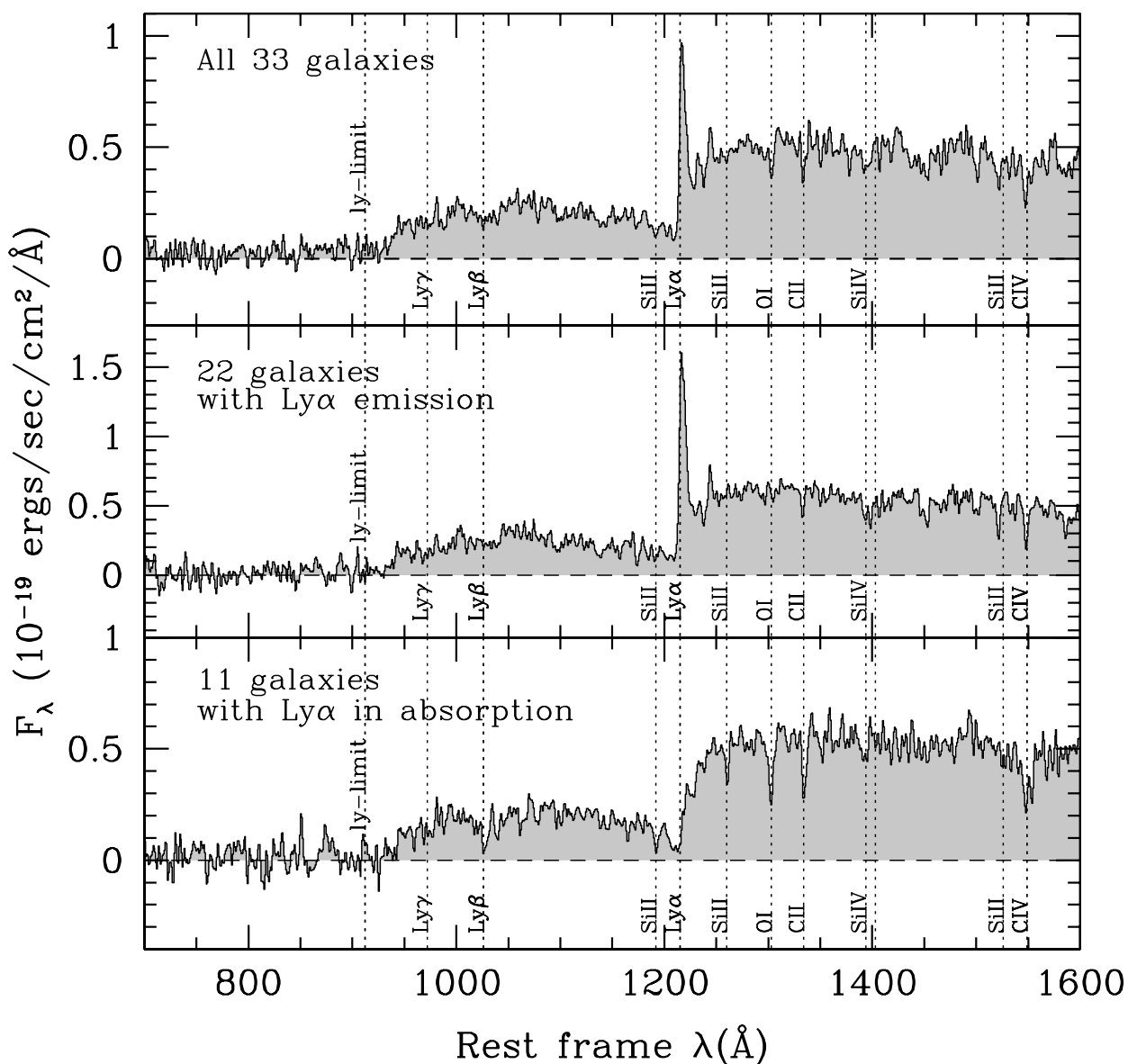
Fig. 22. Average rest-frame spectra ( F_\lambda ) of galaxies with flags 2, 3 and 4 in VUDS with 4.7 \leq z \leq 5.3 : top : stack of all galaxy spectra; middle : stack of galaxies with Ly- \alpha in emission; bottom : stack of galaxies with Ly- \alpha in absorption (this stack is from a subset of the final sample available at the time of writing).
