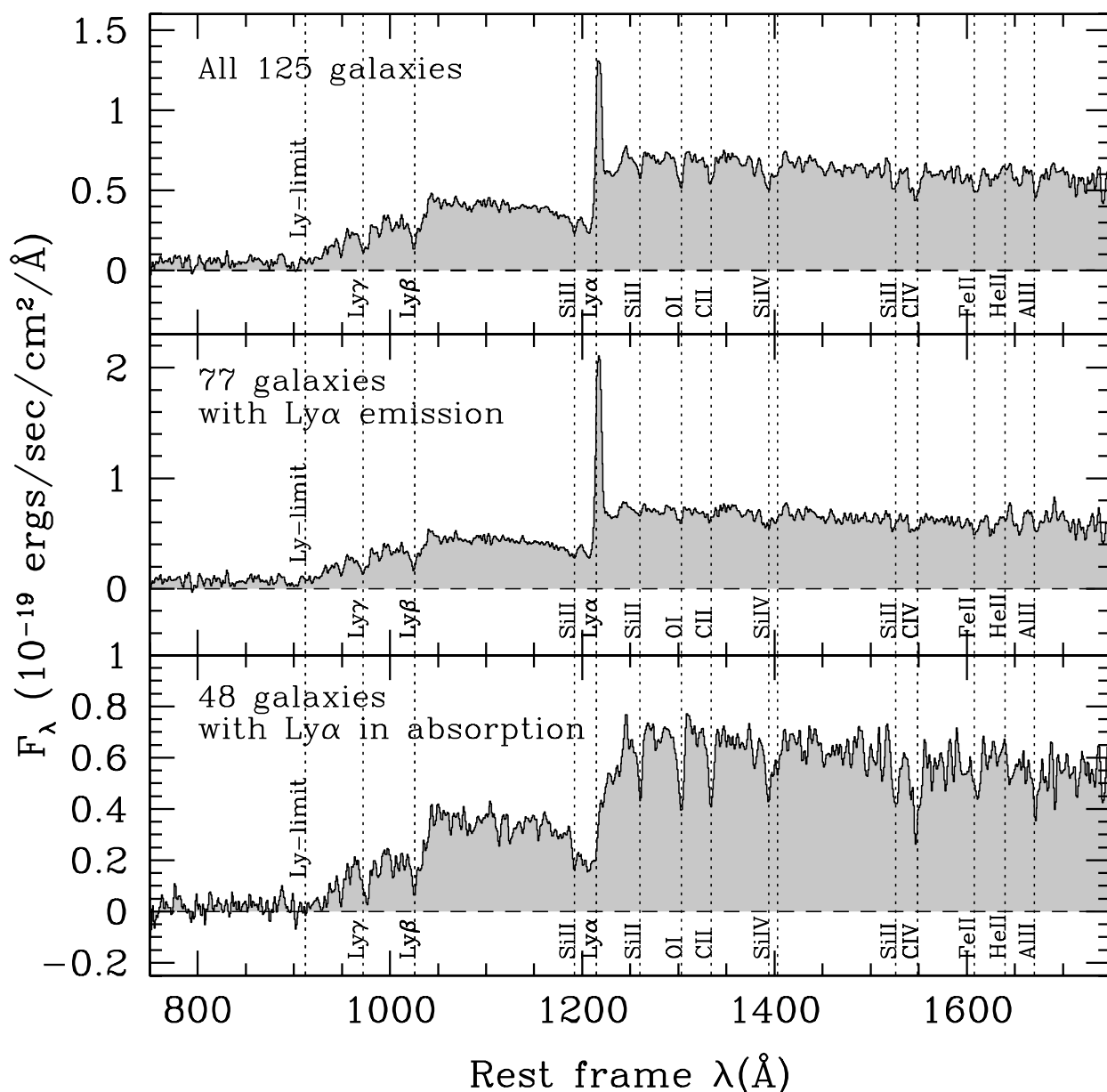
Fig. 21. Average rest-frame spectra ( F_\lambda ) of galaxies with flags 2, 3 and 4 in VUDS with 4 \leq z \leq 4.7 : top : stack of all galaxy spectra; middle : stack of galaxies with Ly- \alpha in emission; bottom : stack of galaxies with Ly- \alpha in absorption (this stack is from a subset of the final sample available at the time of writing).
