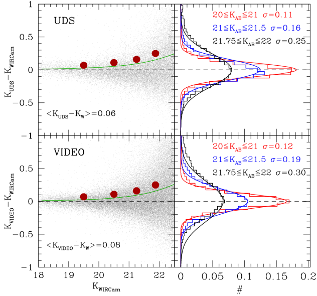
Fig. 4. Comparison of the VIPERS K -band photometry with the Ultra-Deep UKIDSS field ( top left ), the VIDEO XMM2 field ( bottom left ), and the scatter distributions in three magnitude bins ( right panels ). The observed scatters are reported in the left panels as red circles, while the green solid lines show the mean magnitude vs. error behaviour of our VIPERS K band data after rescaling the original errors by 1.5 (see text). Larger dispersions are observed with VIDEO than with UDS because of the different depths between the two fields.
