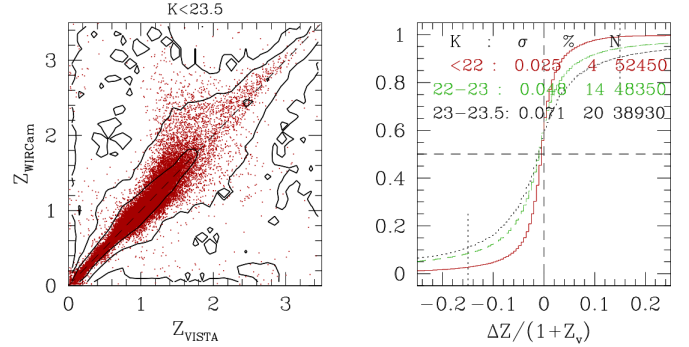
Fig. 13. Comparison of the photometric redshifts measured using either WIRCam K band ( z_{\text{wircam}} ) or YJHK photometry from VISTA ( z_{\text{vista}} ) for galaxies with K_{\text{VISTA}} \leq 23.5 . The left panel shows the comparison z_{\text{wircam}} vs. z_{\text{vista}} for K_{\text{VISTA}} < 22 (red dots), while the density contours spaced in logarithmic scale of 1 dex are for the faint sample, 22 < K_{\text{VISTA}} < 23.5 . The right panel shows the cumulative distributions of the difference ( \Delta z/(1+z_v) ) split into three K -band subsamples ( K_{\text{VISTA}} \leq 22 : red line; 22 < K_{\text{VISTA}} < 23 : green line; 23 < K_{\text{VISTA}} < 23.5 : blue line). We also report the dispersions ( \sigma ), the fractions of catastrophic sources (in %), and the number of sources used.
