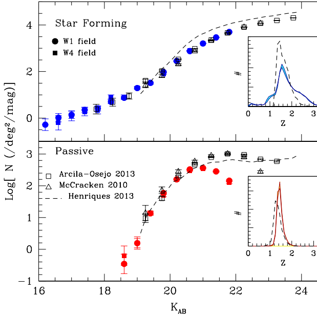
Fig. 15. Differential number counts of star-forming ( top ) and passive ( bottom ) BzK galaxies in the W1 and W4 fields. We compare with deeper observations in CFHTLS deep fields (open squares, Arcila-Osejo & Sawicki 2013) and COSMOS (open triangles, McCracken et al. 2010) and model predictions (dashed lines, Henriques et al. 2013). The inset panels show the photometric redshift distributions with K_{AB} \leq 22 .
