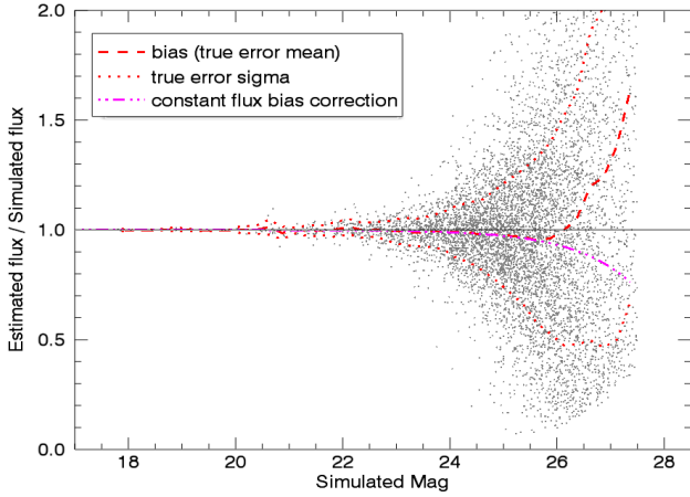
Fig. 6. Comparison of the EM vs. simulated fluxes as a function of simulated magnitudes. The dotted lines show the 1\sigma error, the red dashed line the mean bias. The magenta dot-dashed line reflects the effect of a small background bias on the flux ratio.
