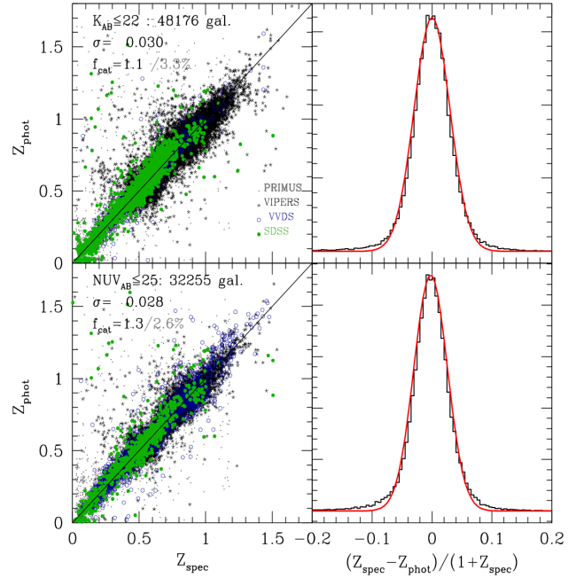
Fig. 11. Comparison of our photometric redshifts with the VVDS, VIPERS, PRIMUS, and BOSS most secure spectroscopic redshifts, for galaxies with K \leq 22 (top panels) and \text{NUV} \leq 25 (bottom panels). We report the dispersion ( \sigma_{\text{NMAD}} ) by combining all the surveys, while the catastrophic fractions ( f_{\text{cat}} defined as |\Delta z|/(1+z_s) > 0.15 ) are given for all surveys but PRIMUS (black value), which is shown separately (gray value). The observed distributions of photometric errors are compared to a Gaussian distribution with the same \sigma (right panels).
