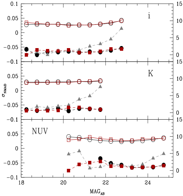
Fig. 12. Comparison of the dispersion ( \sigma_{\text{NMAD}} ) as a function of magnitude (top panel: i ; middle panel: K_s ; bottom panel: NUV). The \sigma_{\text{NMAD}} for the W1 (black circles) and W4 (red squares) fields correspond to the open symbols and solid lines and refer to the left y -axis. The fraction of catastrophic redshifts are reported as field symbols and dashed lines and refer to the right y -axis (%). The PRIMUS spectroscopic sample in W1 field is shown separately (gray triangles).
