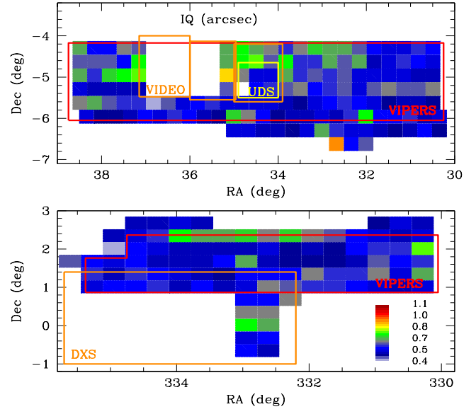
Fig. 2. Colour-coded mean image quality (IQ) per WIRCam tile over the whole WIRCam survey (W1: top and W4: bottom). The layouts indicate the VIPERS regions (red layouts), the three VIDEO pointings (orange in W1), the UKIDSS-UDS (yellow in W1), and UKIDSS-DXS (orange in W4).
