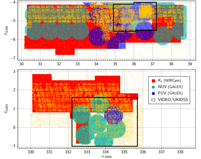
Fig. 1. Footprints of the GALEX NUV/FUV (cyan/blue) and WIRCam K_s band (red background) observations in the CFHTLS W1 (top) and W4 (bottom) fields. The spectroscopic sources are shown as golden points. The total area (W1 and W4) is \sim 7.8 and \sim 22 \text{ deg}^2 in FUV and NUV bands observed with GALEX and \sim 27 \text{ deg}^2 with WIRCam. The black layouts represent the VIDEO (W1) and UKIDSS (W4) surveys.
