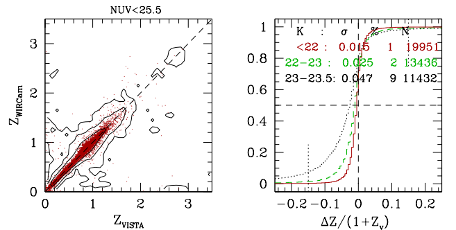
Fig. 14. Same as Fig. 13 for a NUV-selected sample with NUV \leq 25.5 and also split into K_{\text{VISTA}} subsamples.
