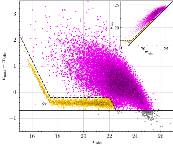
Fig. 9. Photometric classification between point-like and extended sources in the \mu_{\max} - m_{\text{obs}} vs. m_{\text{obs}} plane (for one tile of the CFHTLS in the i -band). The dashed line represents our selection of point-like sources ( S^\mu , yellow dots). All objects lying below the solid line (gray dots) are considered as false detections.
