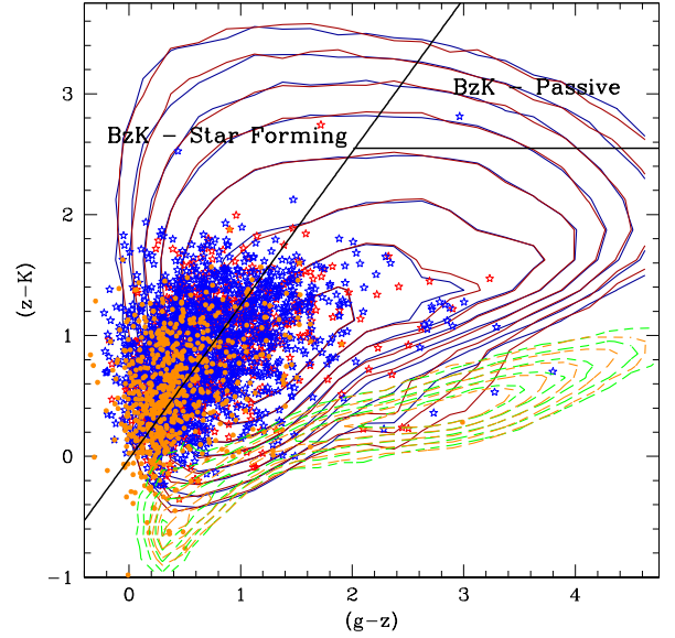
Fig. 10. Distribution of galaxies, stars, and QSOs in the (z - K) vs. (g - z) colour diagram. Density levels are in logarithmic scale ( \Delta = 0.3 dex) for galaxies (solid lines in W1 and W4 fields shown blue and red, respectively) and stars (dashed lines in green and orange). Objects from our QSO samples are shown as open stars (blue: W1; red: W4), while the SDSS/VIPERS AGN sample is shown as orange dots. The solid black lines delineate the high-redshift BzK populations (star-forming and passive galaxies).
