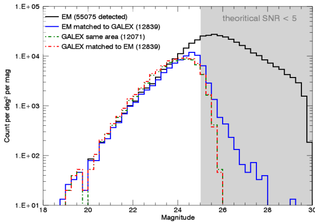
Fig. 7. NUV number counts vs. magnitude in one GALEX field. The full EM photometric catalogue is shown as a solid black line and the EM sources matched to the GALEX pipeline sources as a solid blue line. The GALEX pipeline counts in the same area (and matched to EM sources) are shown as red and green dot-dashed lines.
