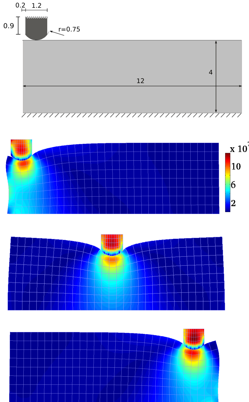
Figure 6: Initial geometry and deformed configuration of the shallow ironing example with contour plot of the Von-Mises stress in the frictionless case, at t = 1 , t = 1.5 and t = 2 .
