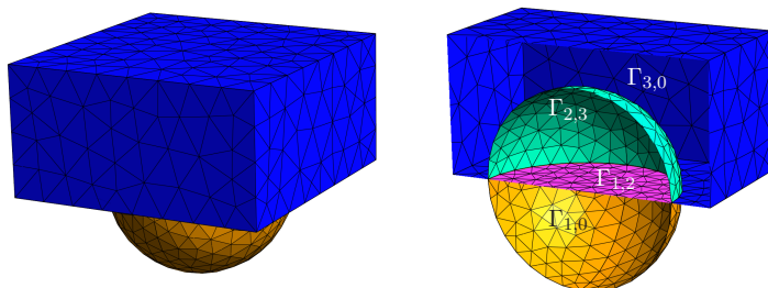
Fig. 5 Experiment II: Geometric setup
