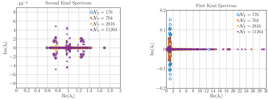
Fig. 3 Experiment I: Spectrum of Galerkin matrices for 2nd-kind (left) and 1st-kind (right) STF
