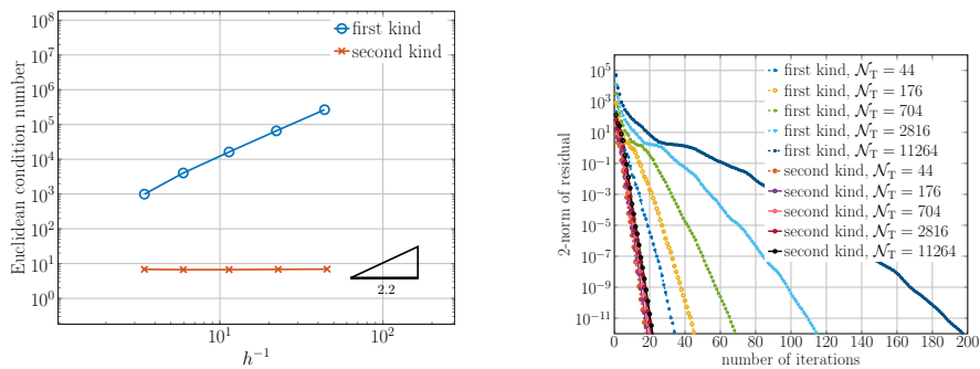
Fig. 4 Experiment I: Euclidean condition numbers (left) and convergence history of GMRES in terms of decrease of Euclidean norm of residual vectors (right)
